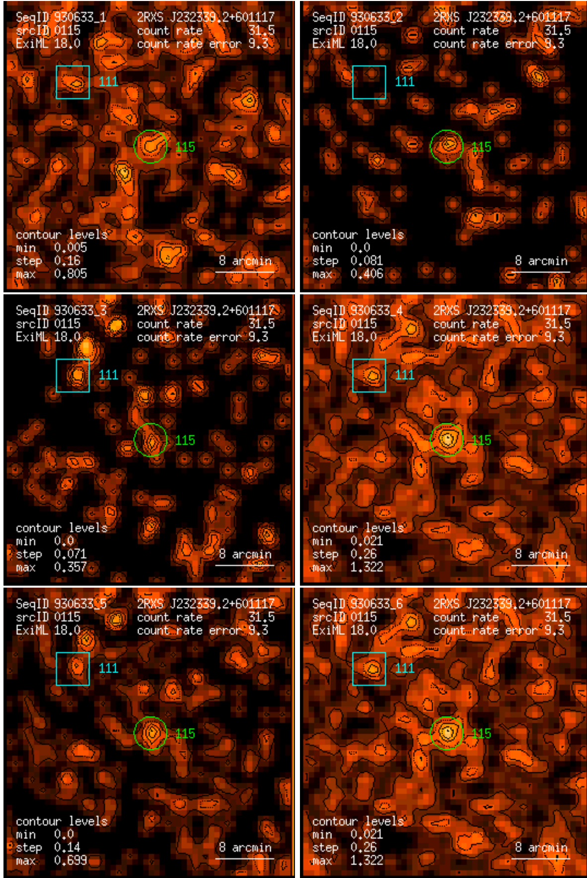
Figure 115: RASS 930633: detection 0115: band rate images, Gaussian filter: (1) PSPC channels 11 – 41, (2) 52 – 90, (3) 91 – 201, (4) 11 – 235, (5) 52 – 201, (6) 11 – 201. Broad band rates in counts/ks. Band rate contour levels in counts/ks/arcmin 2 .
