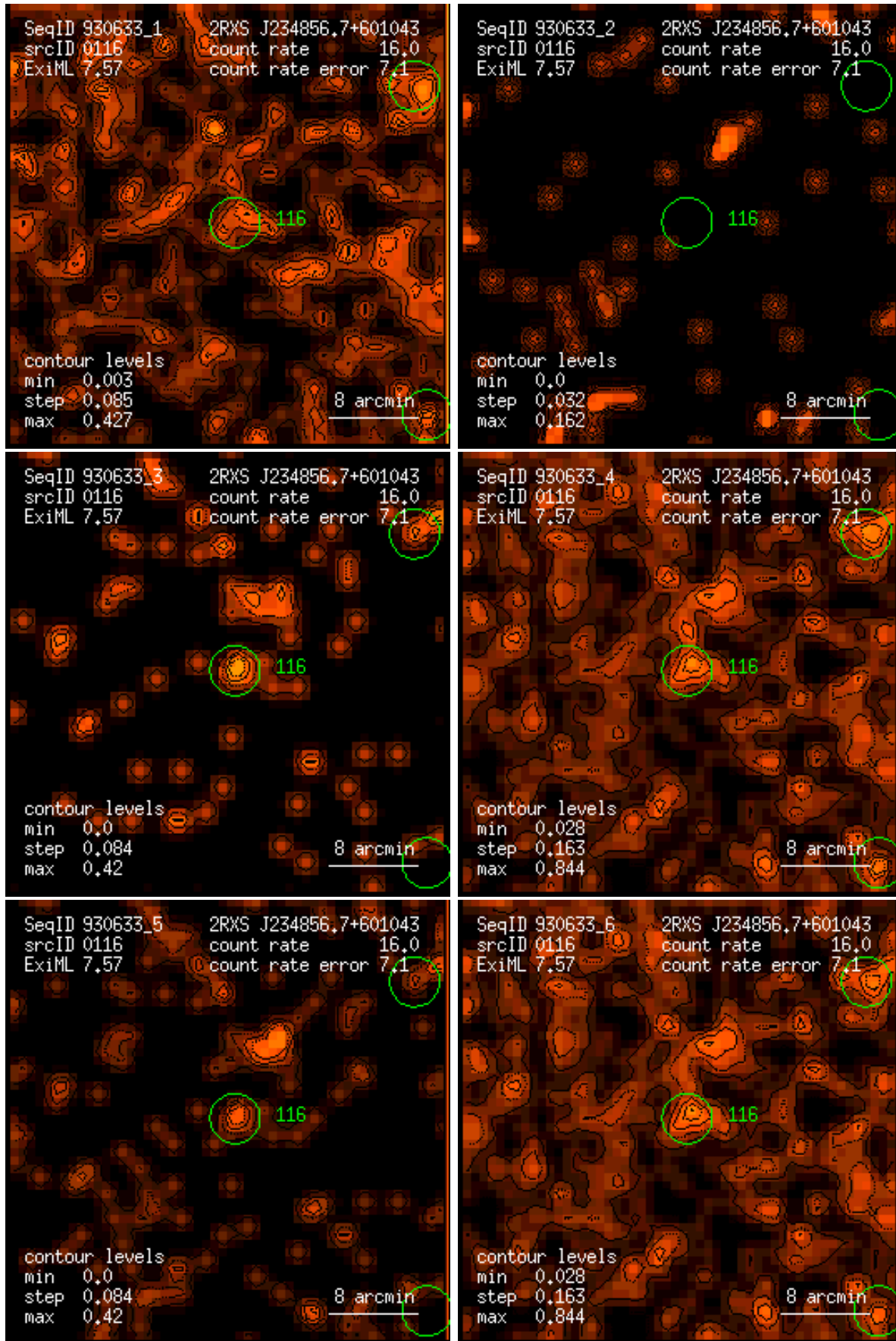
Figure 116: RASS 930633: detection 0116: band rate images, Gaussian filter: (1) PSPC channels 11 – 41, (2) 52 – 90, (3) 91 – 201, (4) 11 – 235, (5) 52 – 201, (6) 11 – 201. Broad band rates in counts/ks. Band rate contour levels in counts/ks/arcmin 2 .
