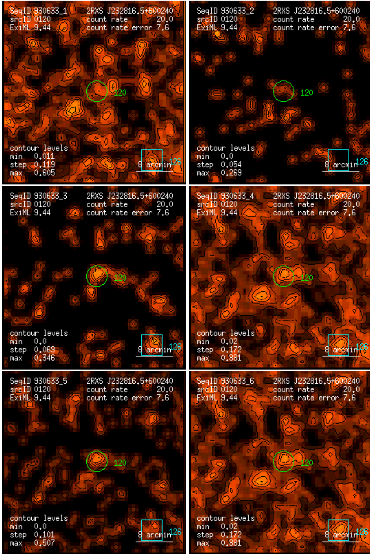
Figure 120: RASS 930633: detection 0120: band rate images, Gaussian filter: (1) PSPC channels 11 – 41, (2) 52 – 90, (3) 91 – 201, (4) 11 – 235, (5) 52 – 201, (6) 11 – 201. Broad band rates in counts/ks. Band rate contour levels in counts/ks/arcmin 2 .
