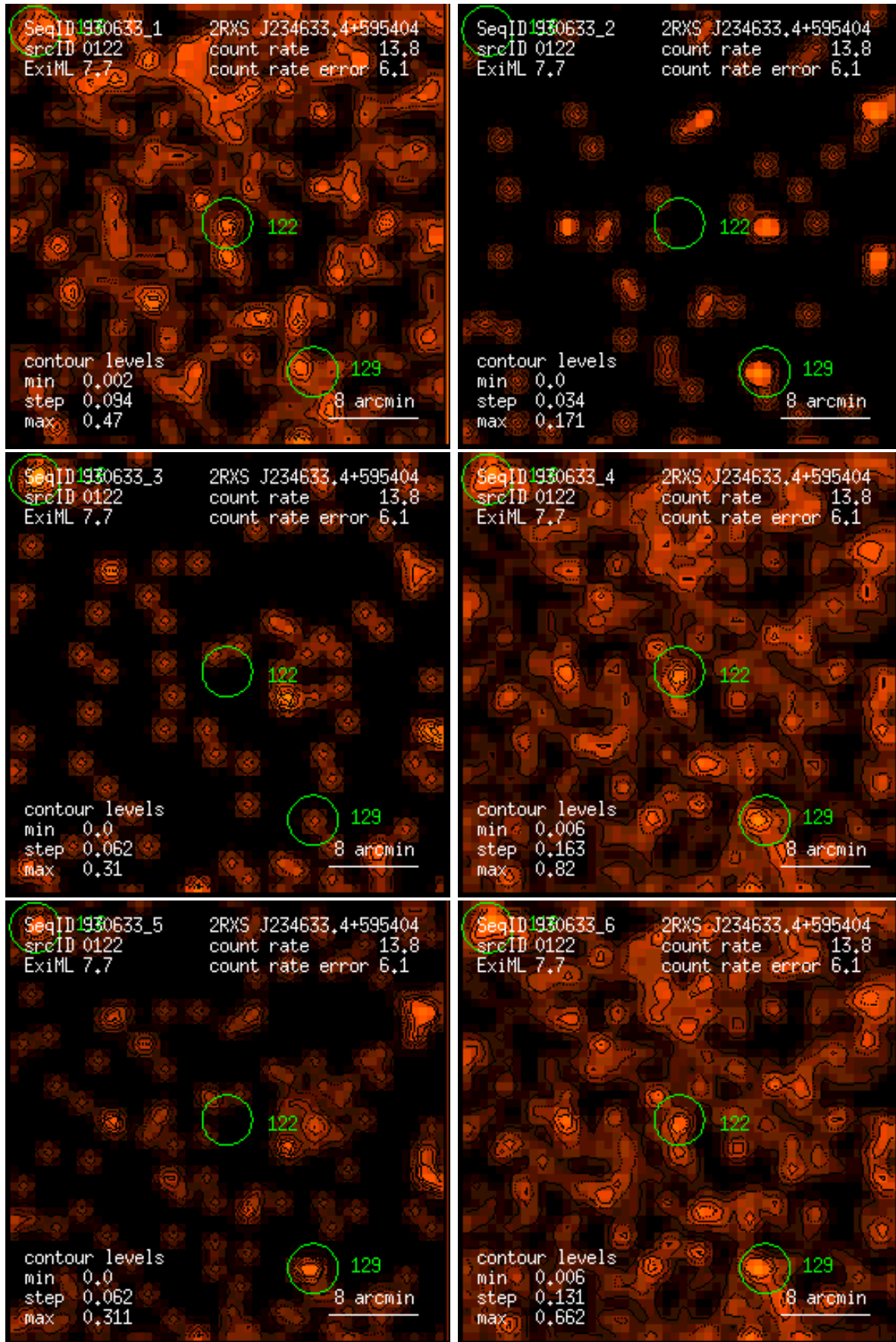
Figure 122: RASS 930633: detection 0122: band rate images, Gaussian filter: (1) PSPC channels 11 – 41, (2) 52 – 90, (3) 91 – 201, (4) 11 – 235, (5) 52 – 201, (6) 11 – 201. Broad band rates in counts/ks. Band rate contour levels in counts/ks/arcmin 2 .
