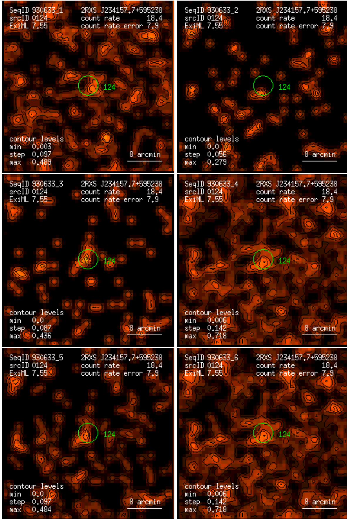
Figure 124: RASS 930633: detection 0124: band rate images, Gaussian filter: (1) PSPC channels 11 – 41, (2) 52 – 90, (3) 91 – 201, (4) 11 – 235, (5) 52 – 201, (6) 11 – 201. Broad band rates in counts/ks. Band rate contour levels in counts/ks/arcmin 2 .
