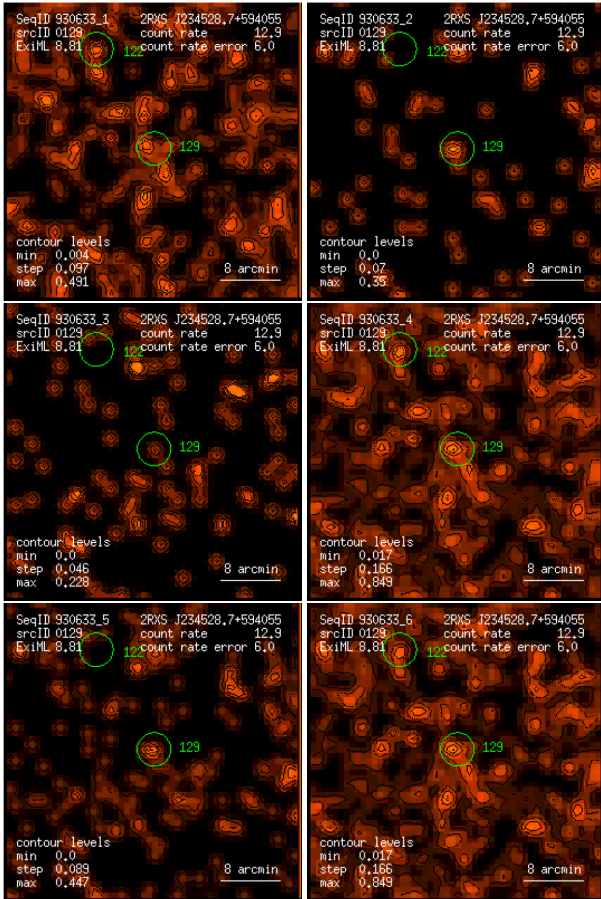
Figure 129: RASS 930633: detection 0129: band rate images, Gaussian filter: (1) PSPC channels 11 – 41, (2) 52 – 90, (3) 91 – 201, (4) 11 – 235, (5) 52 – 201, (6) 11 – 201. Broad band rates in counts/ks. Band rate contour levels in counts/ks/arcmin 2 .
