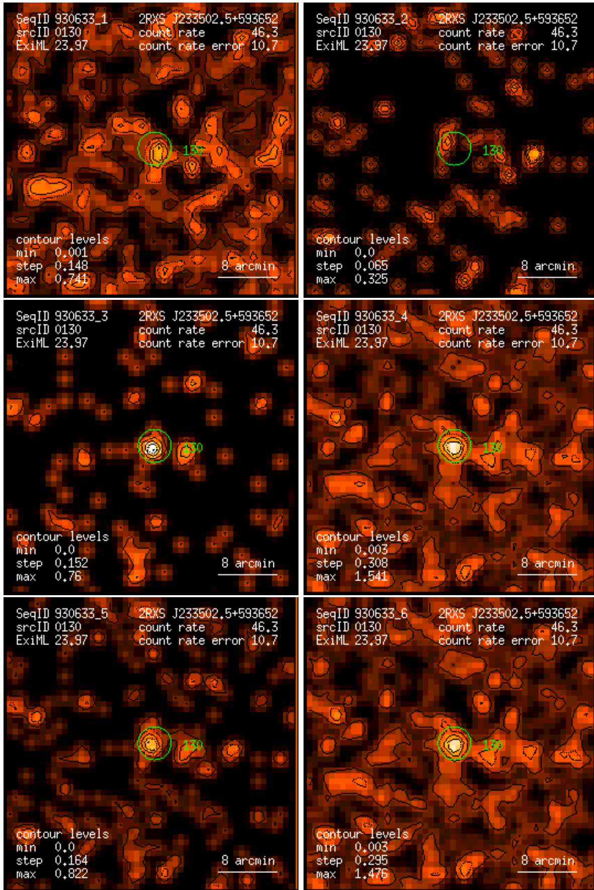
Figure 130: RASS 930633: detection 0130: band rate images, Gaussian filter: (1) PSPC channels 11 – 41, (2) 52 – 90, (3) 91 – 201, (4) 11 – 235, (5) 52 – 201, (6) 11 – 201. Broad band rates in counts/ks. Band rate contour levels in counts/ks/arcmin 2 .
