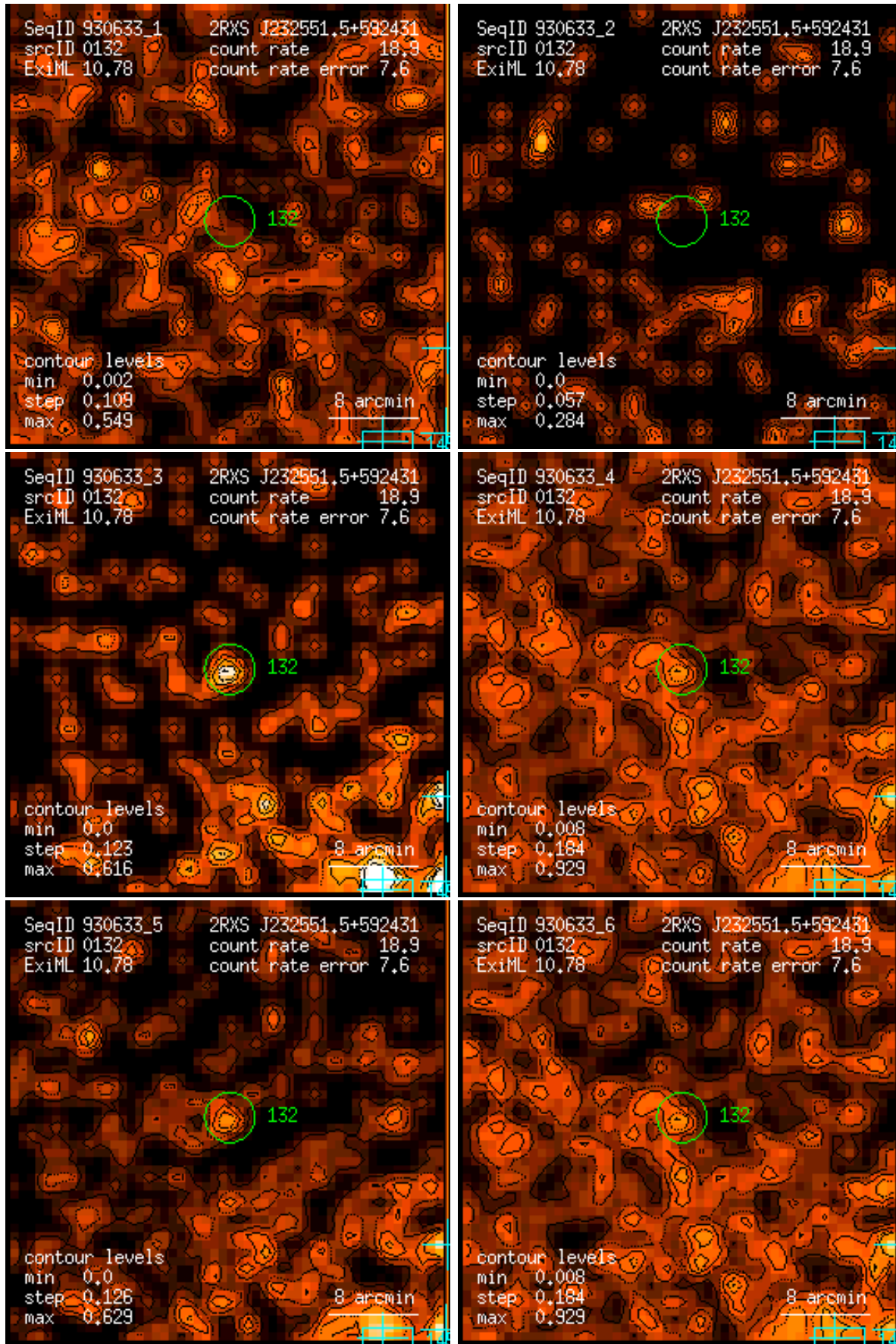
Figure 132: RASS 930633: detection 0132: band rate images, Gaussian filter: (1) PSPC channels 11 – 41, (2) 52 – 90, (3) 91 – 201, (4) 11 – 235, (5) 52 – 201, (6) 11 – 201. Broad band rates in counts/ks. Band rate contour levels in counts/ks/arcmin 2 .
