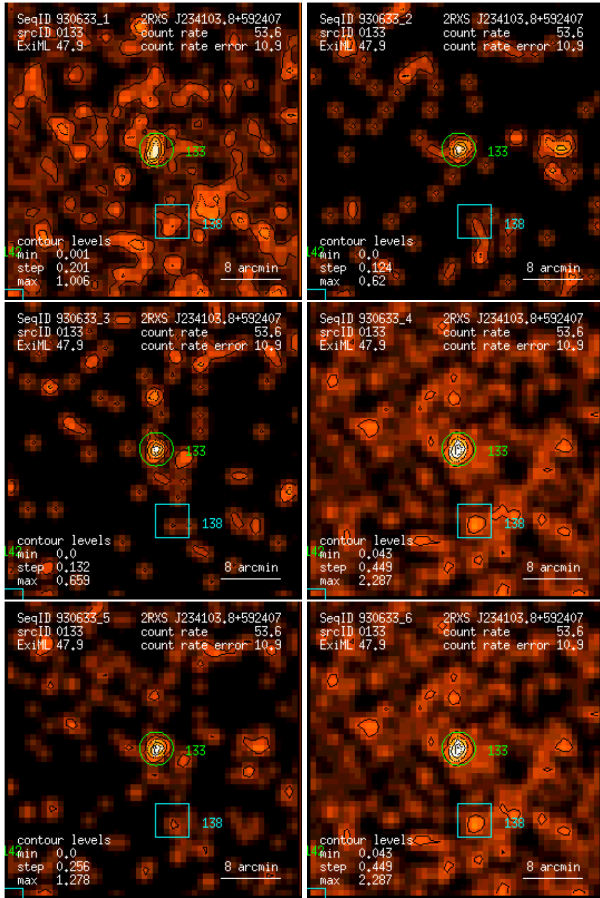
Figure 133: RASS 930633: detection 0133: band rate images, Gaussian filter: (1) PSPC channels 11 – 41, (2) 52 – 90, (3) 91 – 201, (4) 11 – 235, (5) 52 – 201, (6) 11 – 201. Broad band rates in counts/ks. Band rate contour levels in counts/ks/arcmin 2 .
