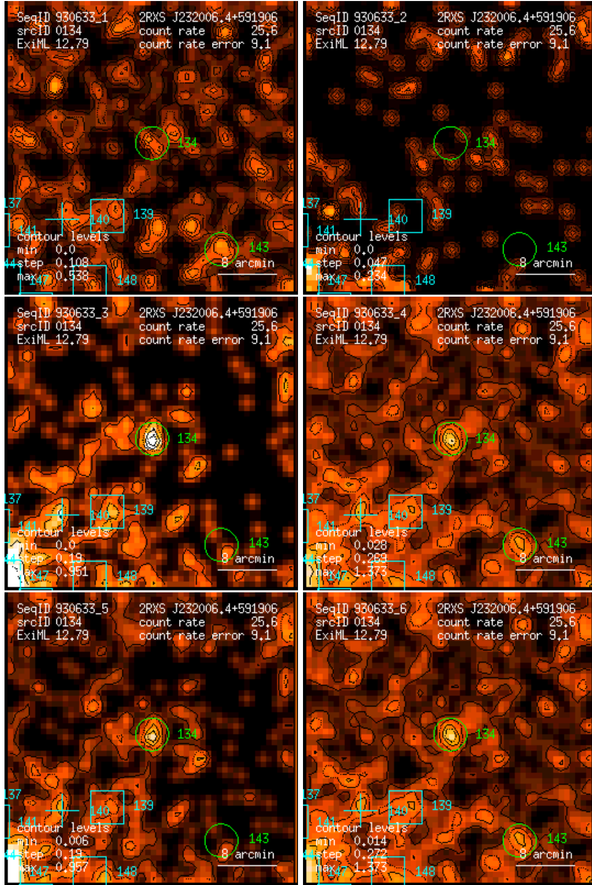
Figure 134: RASS 930633: detection 0134: band rate images, Gaussian filter: (1) PSPC channels 11 – 41, (2) 52 – 90, (3) 91 – 201, (4) 11 – 235, (5) 52 – 201, (6) 11 – 201. Broad band rates in counts/ks. Band rate contour levels in counts/ks/arcmin 2 .
