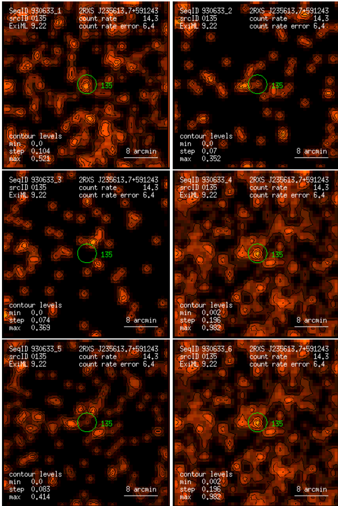
Figure 135: RASS 930633: detection 0135: band rate images, Gaussian filter: (1) PSPC channels 11 – 41, (2) 52 – 90, (3) 91 – 201, (4) 11 – 235, (5) 52 – 201, (6) 11 – 201. Broad band rates in counts/ks. Band rate contour levels in counts/ks/arcmin 2 .
