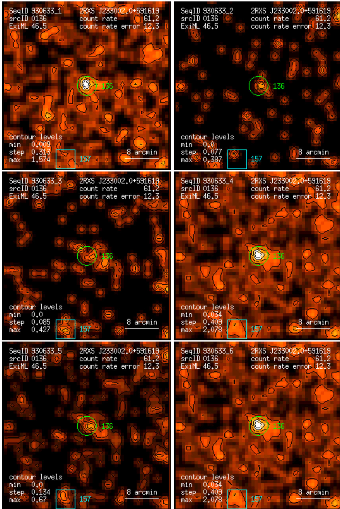
Figure 136: RASS 930633: detection 0136: band rate images, Gaussian filter: (1) PSPC channels 11 – 41, (2) 52 – 90, (3) 91 – 201, (4) 11 – 235, (5) 52 – 201, (6) 11 – 201. Broad band rates in counts/ks. Band rate contour levels in counts/ks/arcmin 2 .
