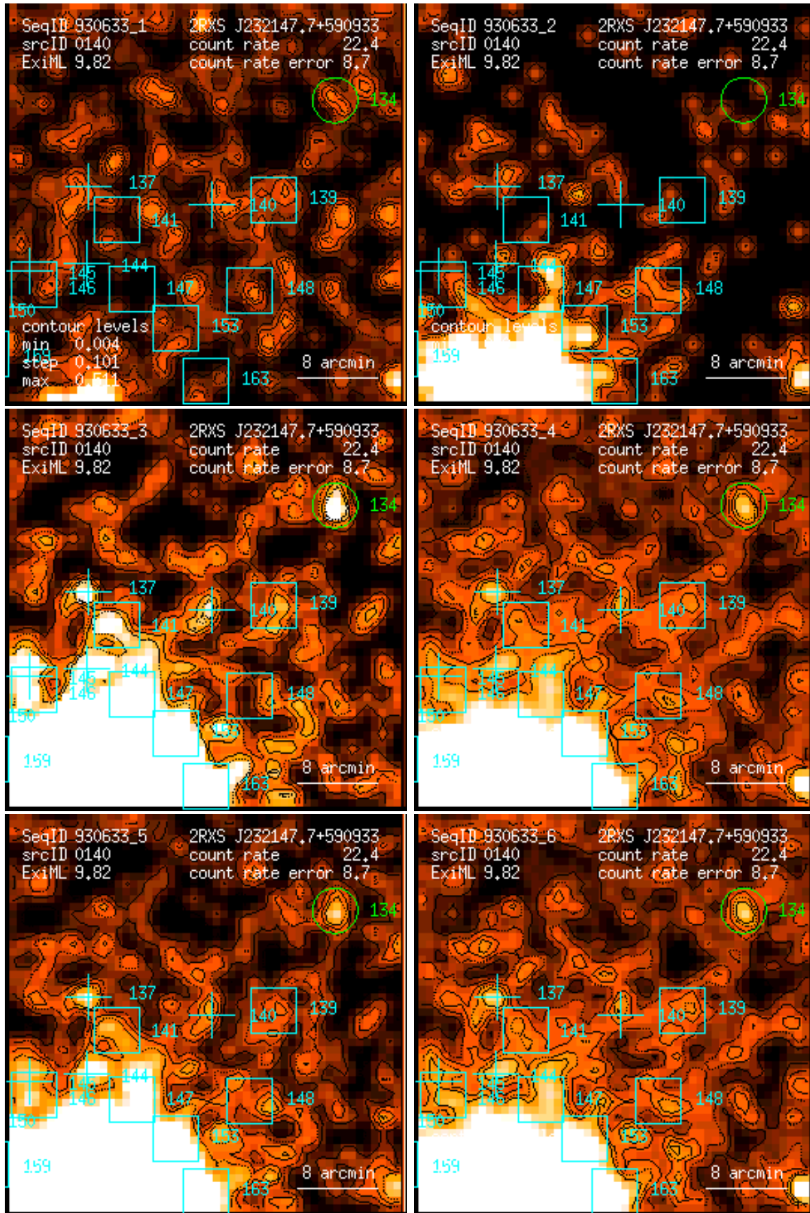
Figure 140: RASS 930633: detection 0140: band rate images, Gaussian filter: (1) PSPC channels 11 – 41, (2) 52 – 90, (3) 91 – 201, (4) 11 – 235, (5) 52 – 201, (6) 11 – 201. Broad band rates in counts/ks. Band rate contour levels in counts/ks/arcmin 2 .
