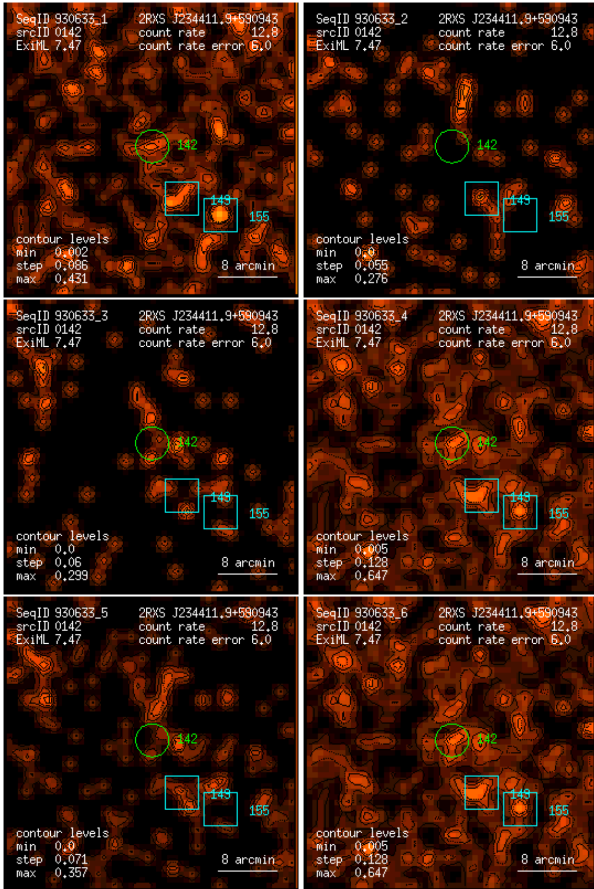
Figure 142: RASS 930633: detection 0142: band rate images, Gaussian filter: (1) PSPC channels 11 – 41, (2) 52 – 90, (3) 91 – 201, (4) 11 – 235, (5) 52 – 201, (6) 11 – 201. Broad band rates in counts/ks. Band rate contour levels in counts/ks/arcmin 2 .
