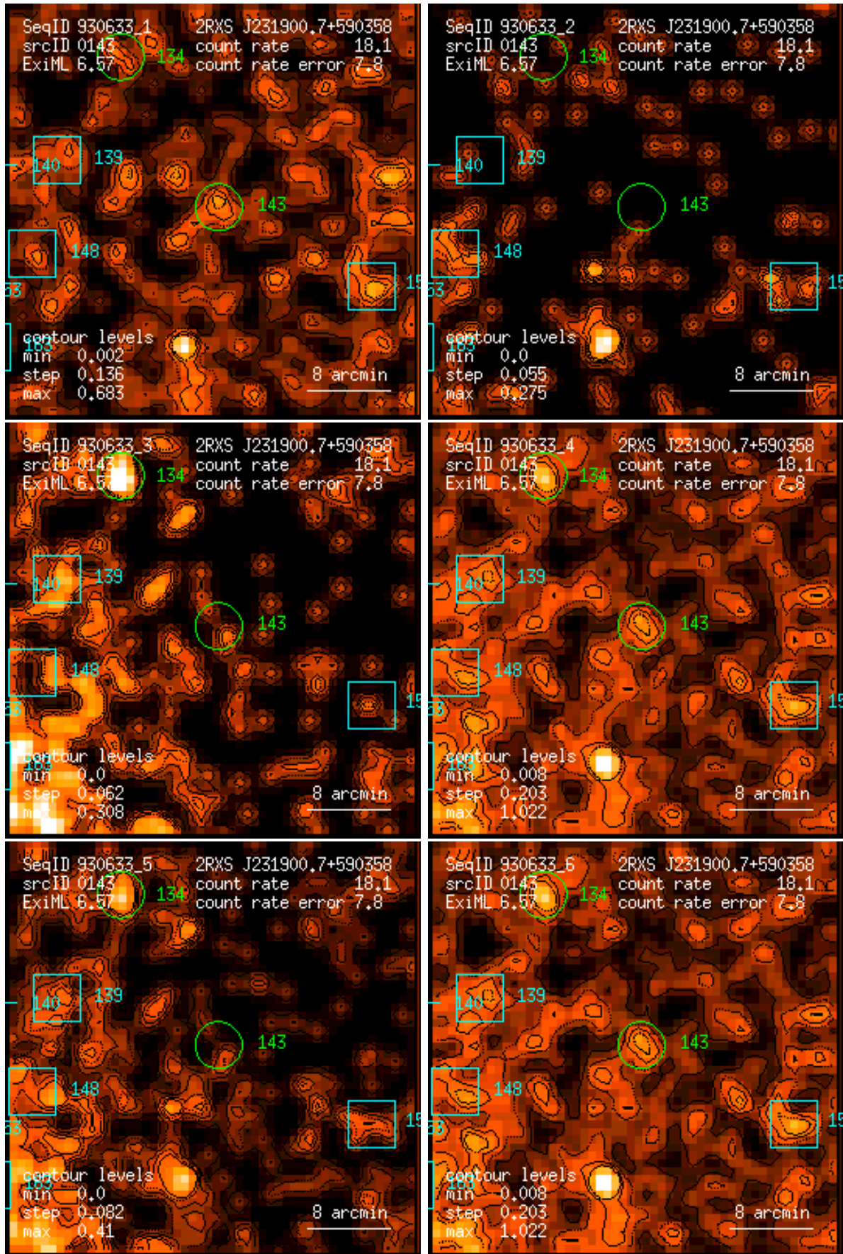
Figure 143: RASS 930633: detection 0143: band rate images, Gaussian filter: (1) PSPC channels 11 – 41, (2) 52 – 90, (3) 91 – 201, (4) 11 – 235, (5) 52 – 201, (6) 11 – 201. Broad band rates in counts/ks. Band rate contour levels in counts/ks/arcmin 2 .
