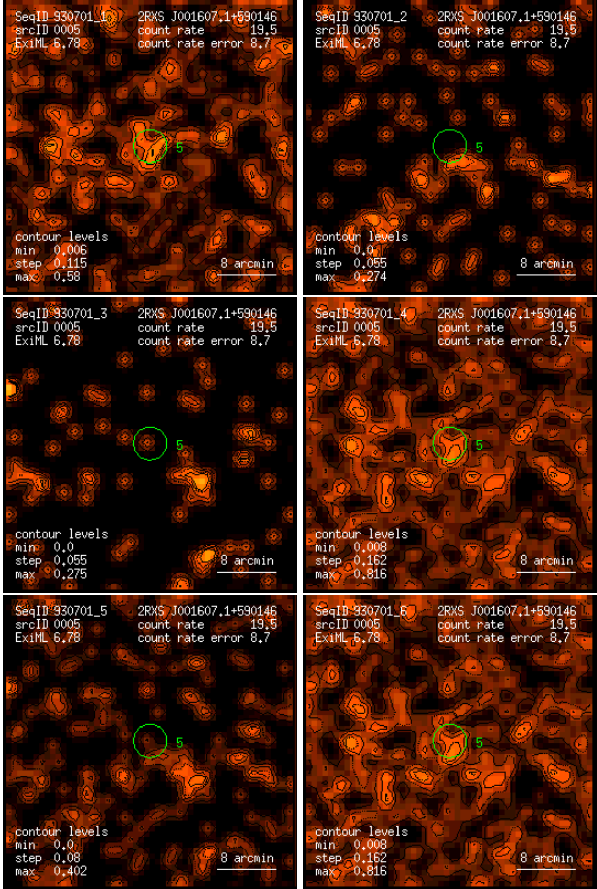
Figure 5: RASS 930701: detection 0005: band rate images, Gaussian filter: (1) PSPC channels 11 – 41, (2) 52 – 90, (3) 91 – 201, (4) 11 – 235, (5) 52 – 201, (6) 11 – 201. Broad band rates in counts/ks. Band rate contour levels in counts/ks/arcmin 2 .
