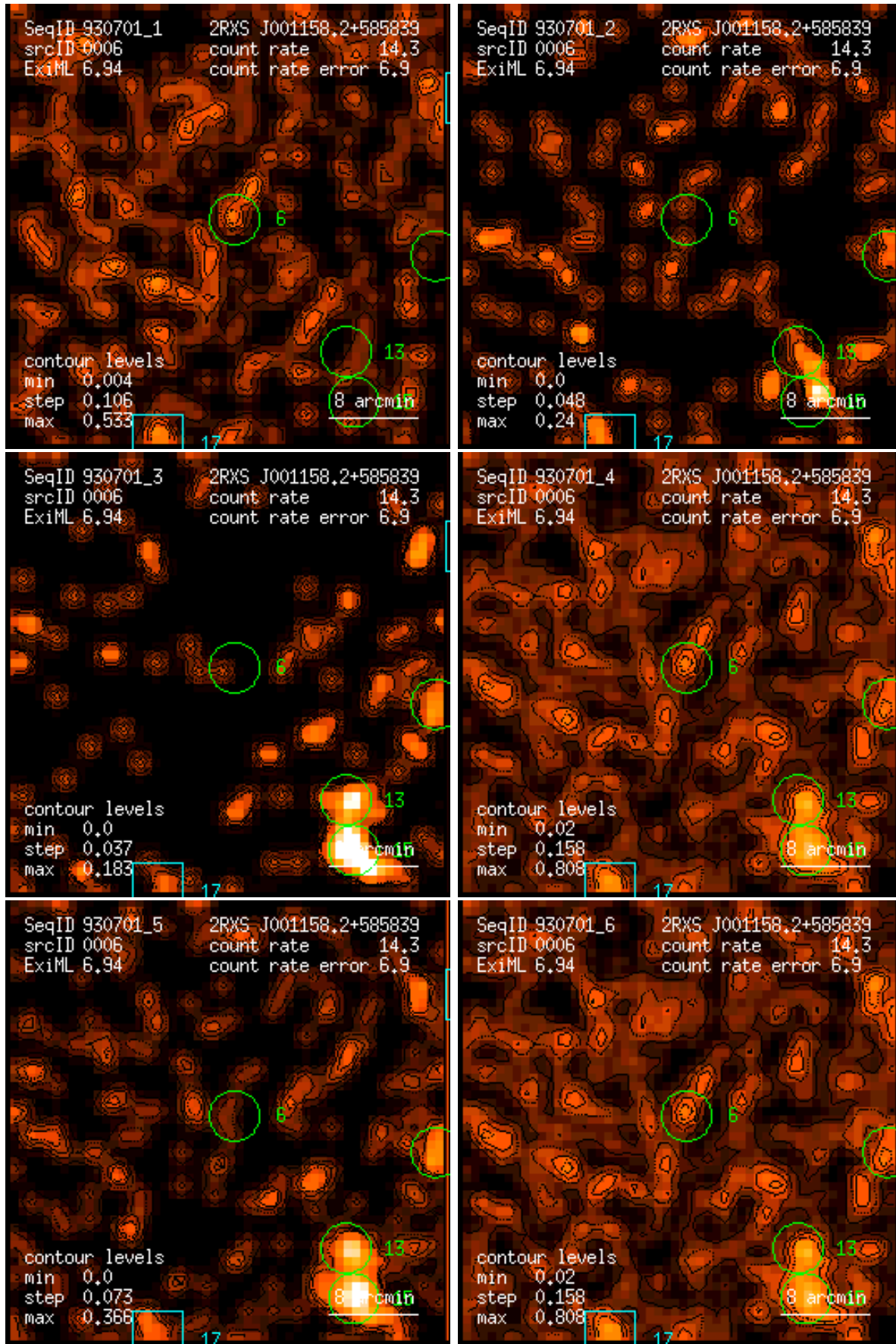
Figure 6: RASS 930701: detection 0006: band rate images, Gaussian filter: (1) PSPC channels 11 – 41, (2) 52 – 90, (3) 91 – 201, (4) 11 – 235, (5) 52 – 201, (6) 11 – 201. Broad band rates in counts/ks. Band rate contour levels in counts/ks/arcmin 2 .
