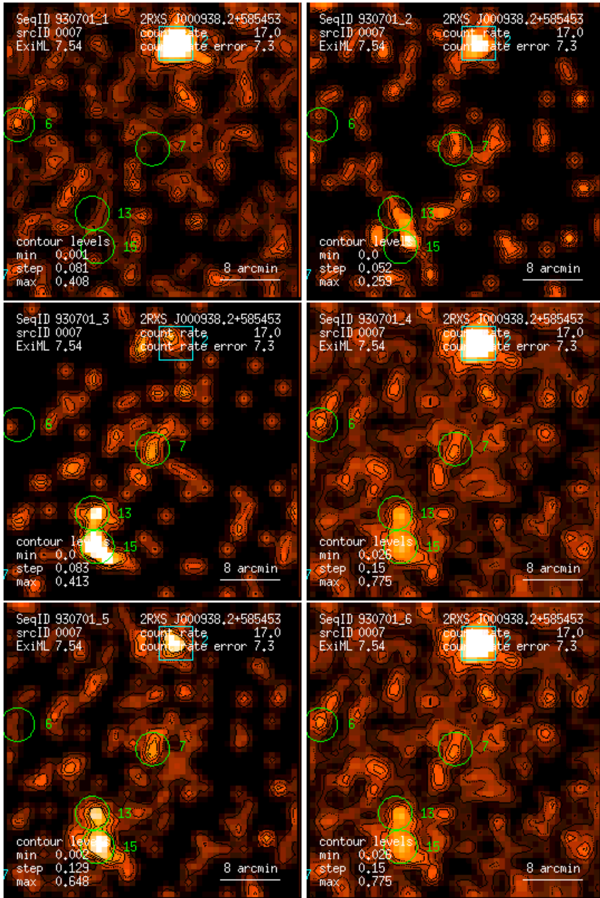
Figure 7: RASS 930701: detection 0007: band rate images, Gaussian filter: (1) PSPC channels 11 – 41, (2) 52 – 90, (3) 91 – 201, (4) 11 – 235, (5) 52 – 201, (6) 11 – 201. Broad band rates in counts/ks. Band rate contour levels in counts/ks/arcmin 2 .
