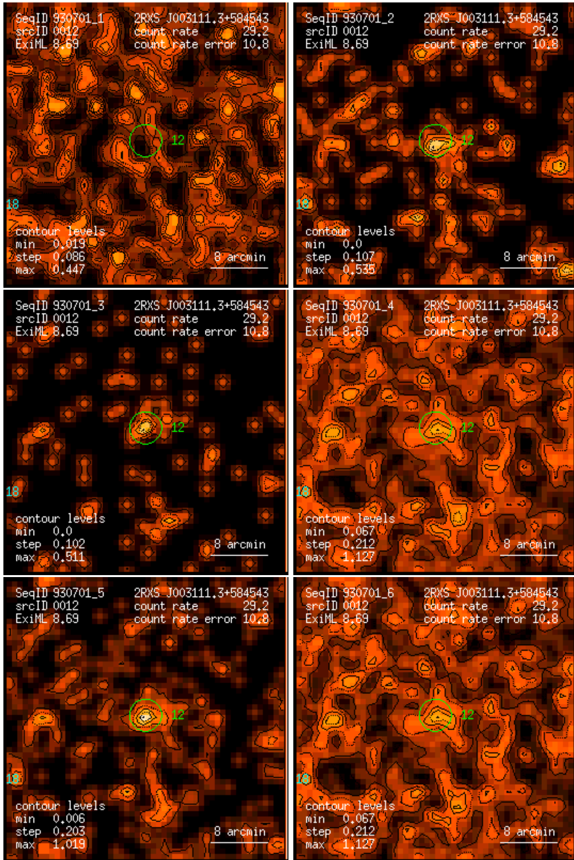
Figure 12: RASS 930701: detection 0012: band rate images, Gaussian filter: (1) PSPC channels 11 – 41, (2) 52 – 90, (3) 91 – 201, (4) 11 – 235, (5) 52 – 201, (6) 11 – 201. Broad band rates in counts/ks. Band rate contour levels in counts/ks/arcmin 2 .
