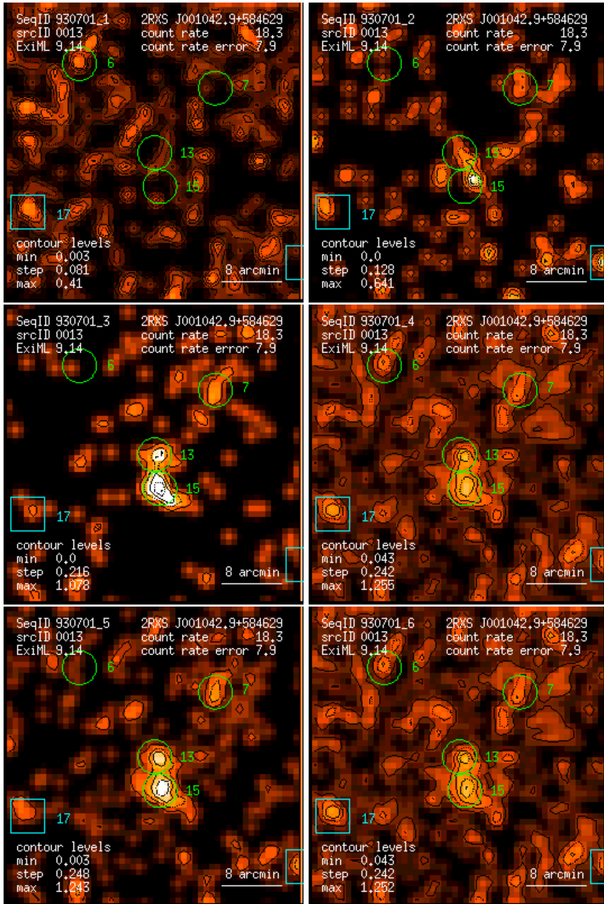
Figure 13: RASS 930701: detection 0013: band rate images, Gaussian filter: (1) PSPC channels 11 – 41, (2) 52 – 90, (3) 91 – 201, (4) 11 – 235, (5) 52 – 201, (6) 11 – 201. Broad band rates in counts/ks. Band rate contour levels in counts/ks/arcmin 2 .
