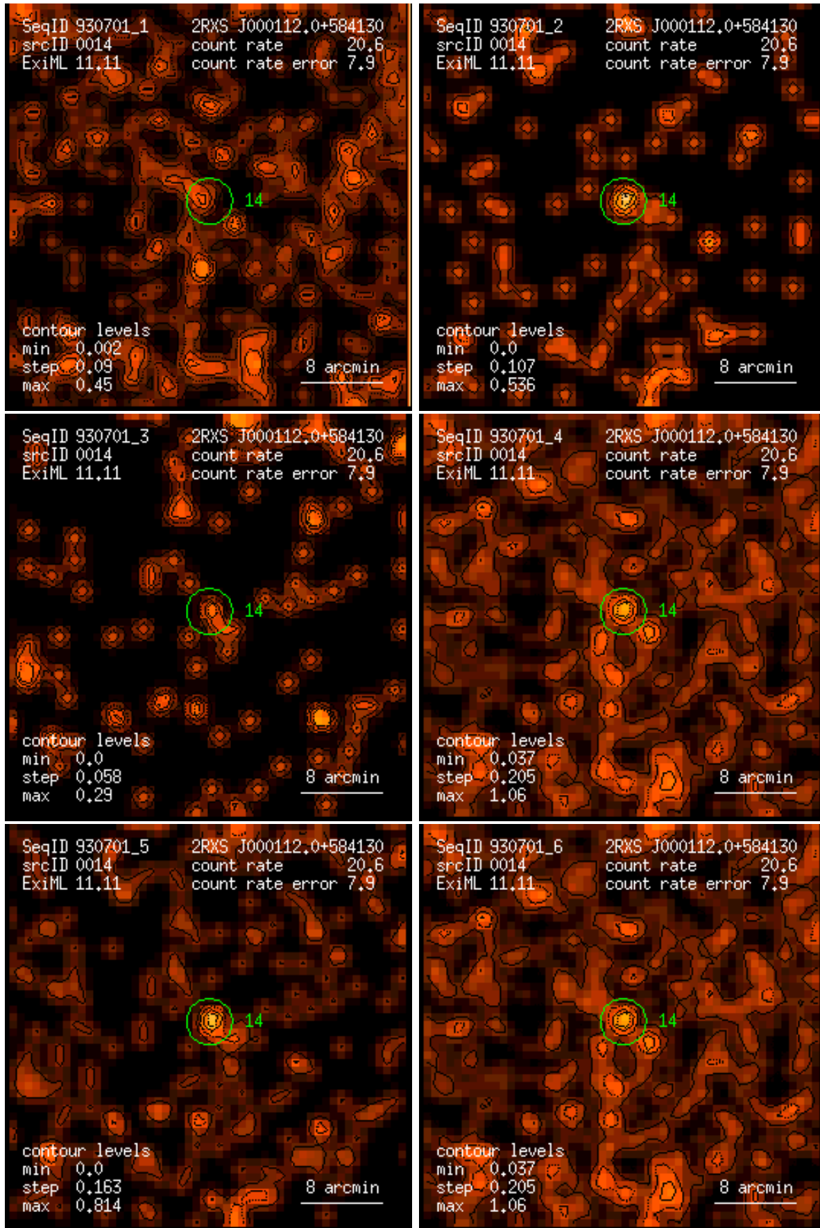
Figure 14: RASS 930701: detection 0014: band rate images, Gaussian filter: (1) PSPC channels 11 – 41, (2) 52 – 90, (3) 91 – 201, (4) 11 – 235, (5) 52 – 201, (6) 11 – 201. Broad band rates in counts/ks. Band rate contour levels in counts/ks/arcmin 2 .
