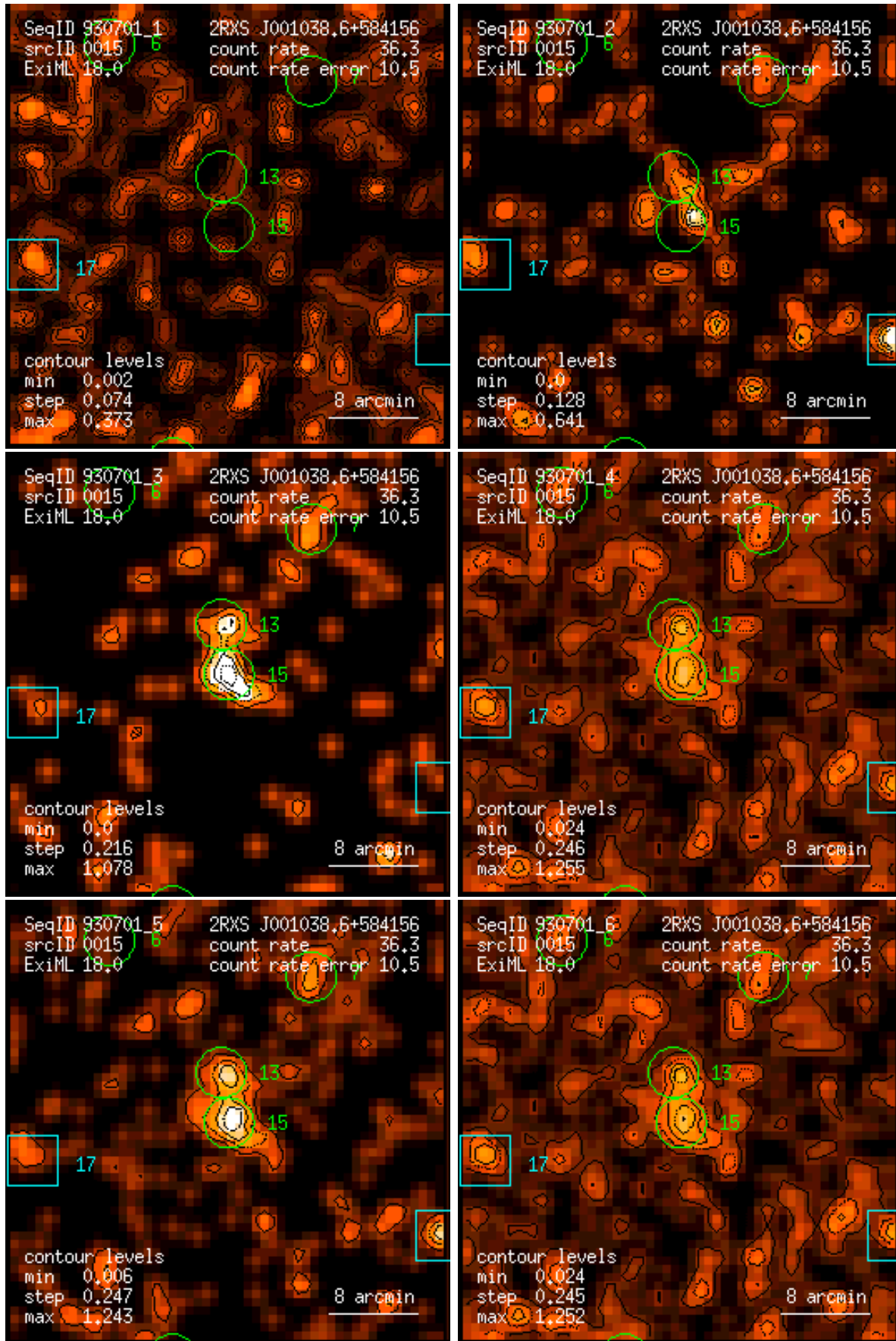
Figure 15: RASS 930701: detection 0015: band rate images, Gaussian filter: (1) PSPC channels 11 – 41, (2) 52 – 90, (3) 91 – 201, (4) 11 – 235, (5) 52 – 201, (6) 11 – 201. Broad band rates in counts/ks. Band rate contour levels in counts/ks/arcmin 2 .
