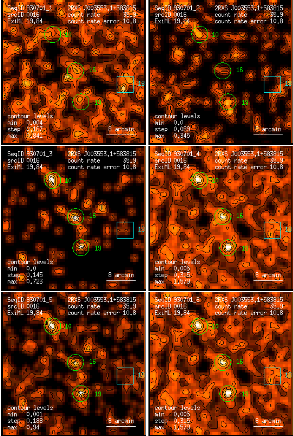
Figure 16: RASS 930701: detection 0016: band rate images, Gaussian filter: (1) PSPC channels 11 – 41, (2) 52 – 90, (3) 91 – 201, (4) 11 – 235, (5) 52 – 201, (6) 11 – 201. Broad band rates in counts/ks. Band rate contour levels in counts/ks/arcmin 2 .
