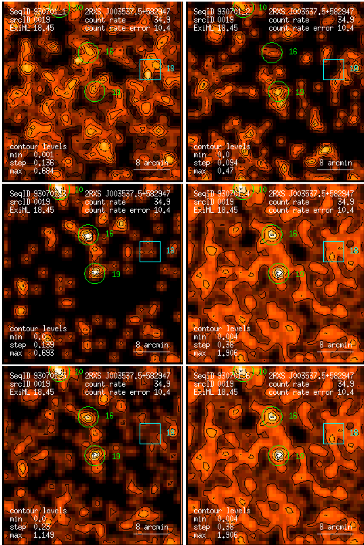
Figure 19: RASS 930701: detection 0019: band rate images, Gaussian filter: (1) PSPC channels 11 – 41, (2) 52 – 90, (3) 91 – 201, (4) 11 – 235, (5) 52 – 201, (6) 11 – 201. Broad band rates in counts/ks. Band rate contour levels in counts/ks/arcmin 2 .
