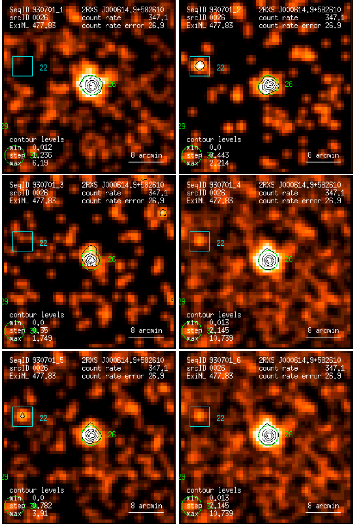
Figure 26: RASS 930701: detection 0026: band rate images, Gaussian filter: (1) PSPC channels 11 – 41, (2) 52 – 90, (3) 91 – 201, (4) 11 – 235, (5) 52 – 201, (6) 11 – 201. Broad band rates in counts/ks. Band rate contour levels in counts/ks/arcmin 2 .
