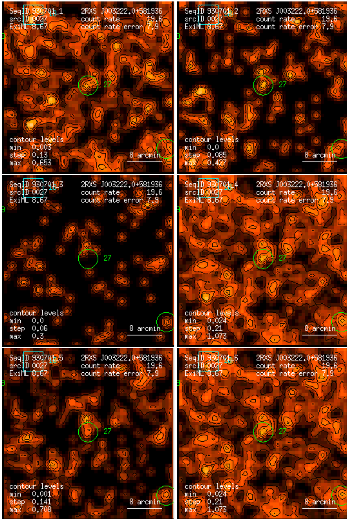
Figure 27: RASS 930701: detection 0027: band rate images, Gaussian filter: (1) PSPC channels 11 – 41, (2) 52 – 90, (3) 91 – 201, (4) 11 – 235, (5) 52 – 201, (6) 11 – 201. Broad band rates in counts/ks. Band rate contour levels in counts/ks/arcmin 2 .
