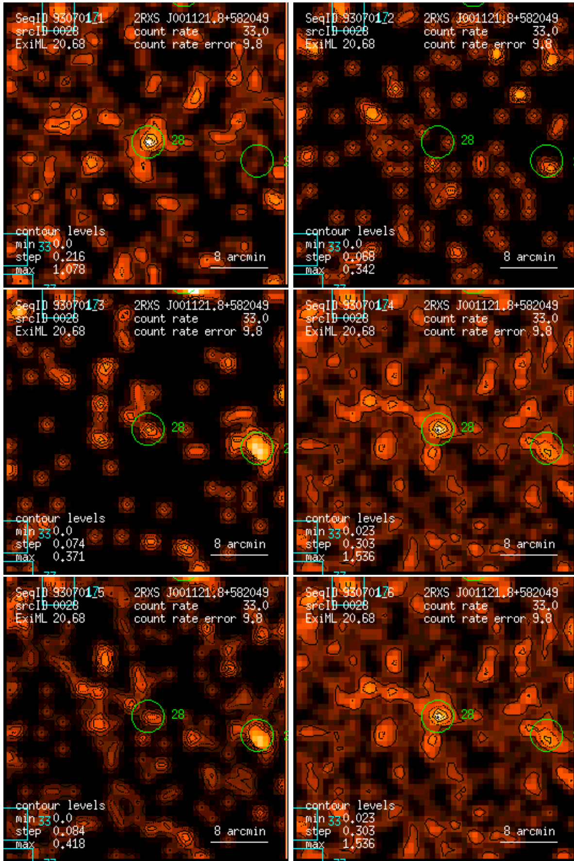
Figure 28: RASS 930701: detection 0028: band rate images, Gaussian filter: (1) PSPC channels 11 – 41, (2) 52 – 90, (3) 91 – 201, (4) 11 – 235, (5) 52 – 201, (6) 11 – 201. Broad band rates in counts/ks. Band rate contour levels in counts/ks/arcmin 2 .
