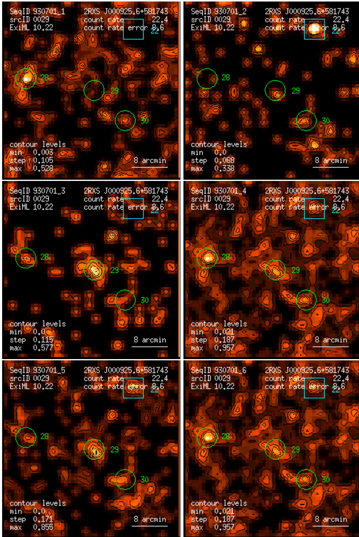
Figure 29: RASS 930701: detection 0029: band rate images, Gaussian filter: (1) PSPC channels 11 – 41, (2) 52 – 90, (3) 91 – 201, (4) 11 – 235, (5) 52 – 201, (6) 11 – 201. Broad band rates in counts/ks. Band rate contour levels in counts/ks/arcmin 2 .
