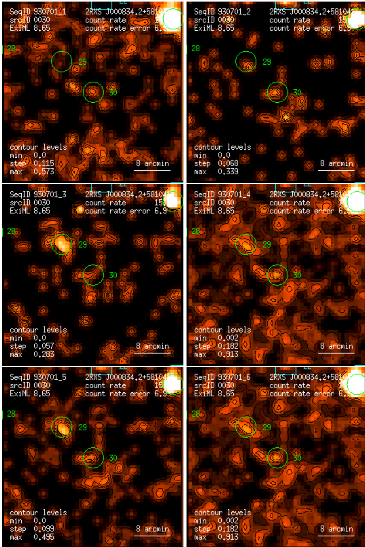
Figure 30: RASS 930701: detection 0030: band rate images, Gaussian filter: (1) PSPC channels 11 – 41, (2) 52 – 90, (3) 91 – 201, (4) 11 – 235, (5) 52 – 201, (6) 11 – 201. Broad band rates in counts/ks. Band rate contour levels in counts/ks/arcmin 2 .
