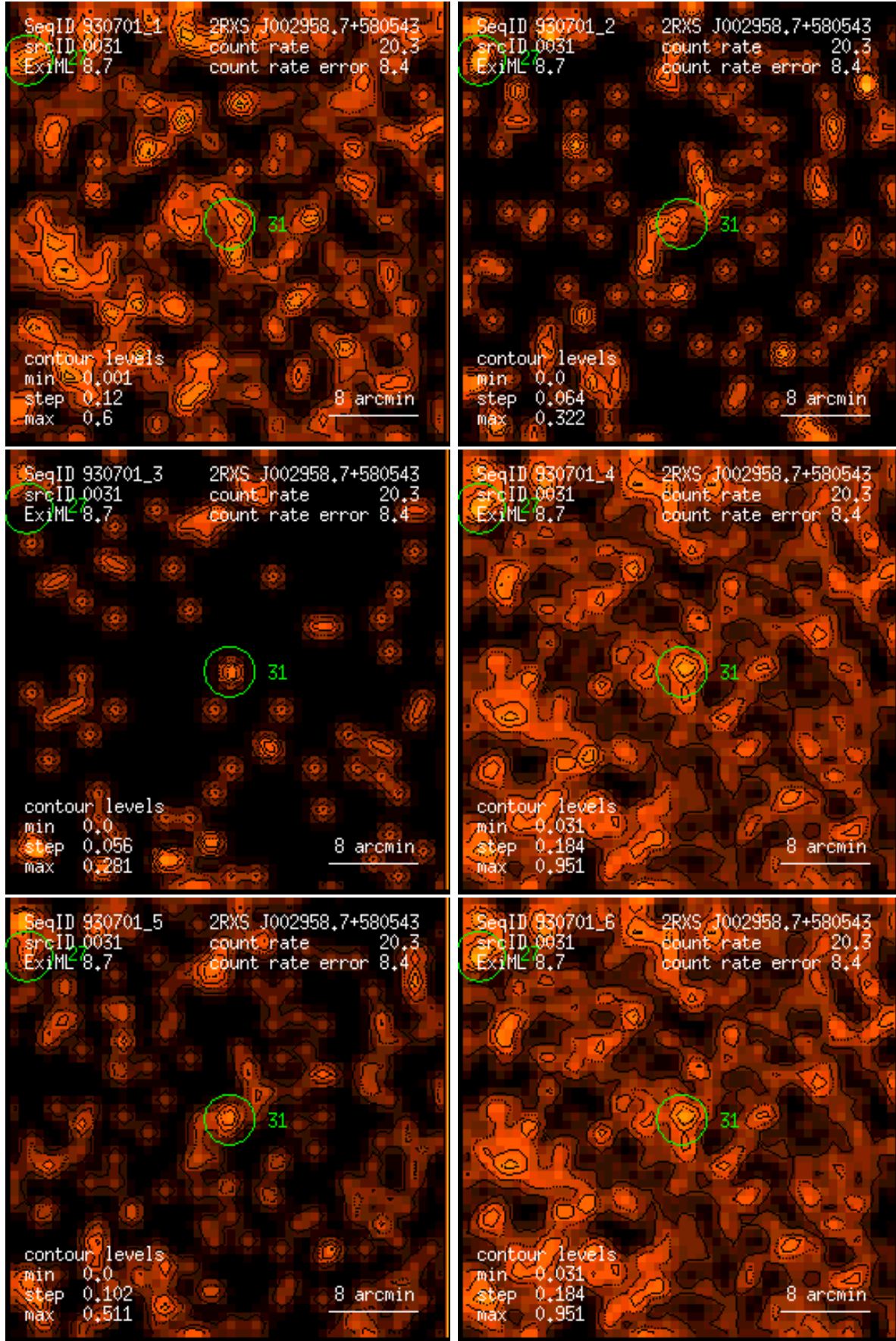
Figure 31: RASS 930701: detection 0031: band rate images, Gaussian filter: (1) PSPC channels 11 – 41, (2) 52 – 90, (3) 91 – 201, (4) 11 – 235, (5) 52 – 201, (6) 11 – 201. Broad band rates in counts/ks. Band rate contour levels in counts/ks/arcmin 2 .
