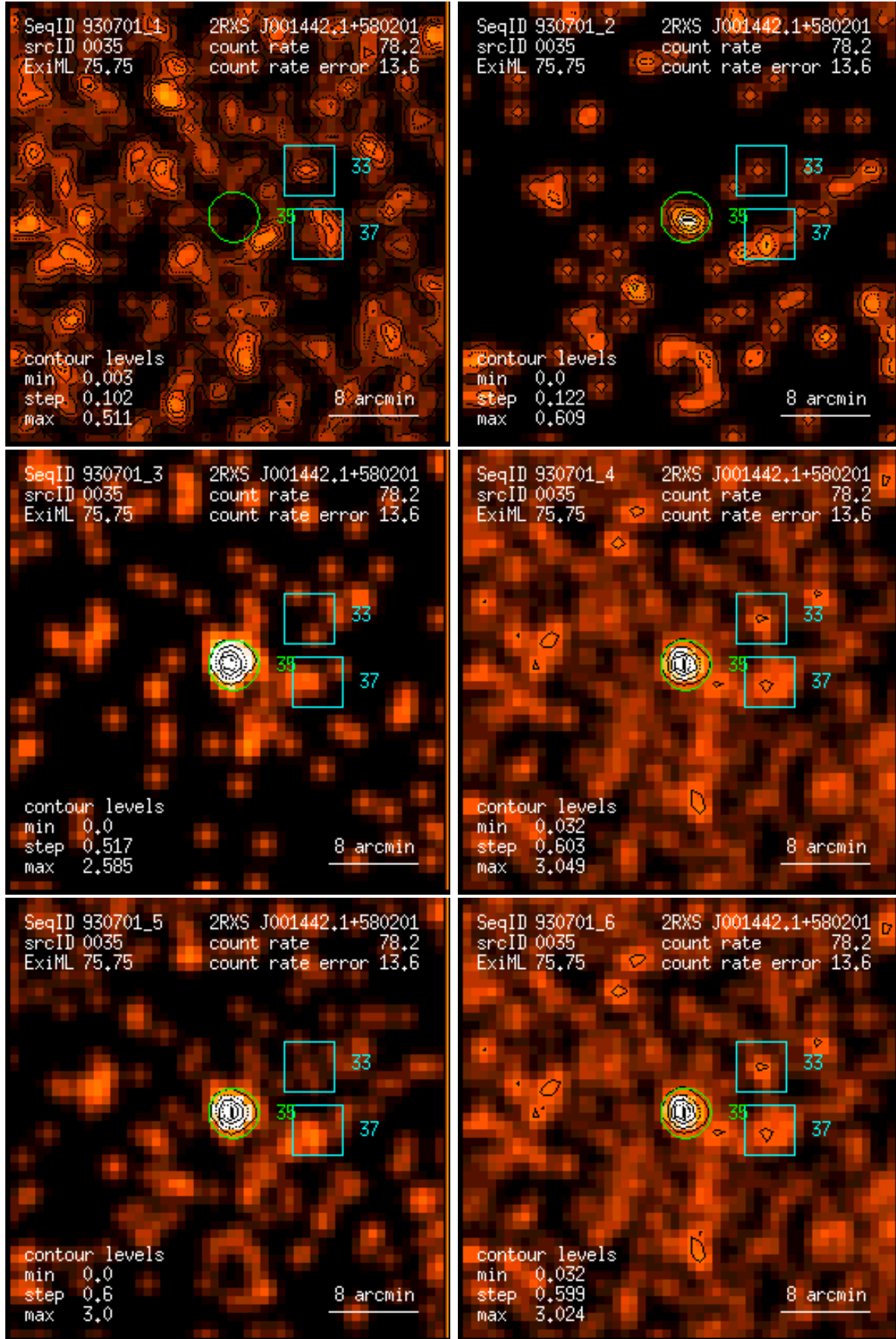
Figure 35: RASS 930701: detection 0035: band rate images, Gaussian filter: (1) PSPC channels 11 – 41, (2) 52 – 90, (3) 91 – 201, (4) 11 – 235, (5) 52 – 201, (6) 11 – 201. Broad band rates in counts/ks. Band rate contour levels in counts/ks/arcmin 2 .
