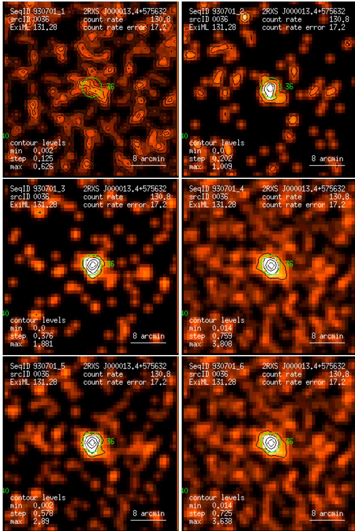
Figure 36: RASS 930701: detection 0036: band rate images, Gaussian filter: (1) PSPC channels 11 – 41, (2) 52 – 90, (3) 91 – 201, (4) 11 – 235, (5) 52 – 201, (6) 11 – 201. Broad band rates in counts/ks. Band rate contour levels in counts/ks/arcmin 2 .
