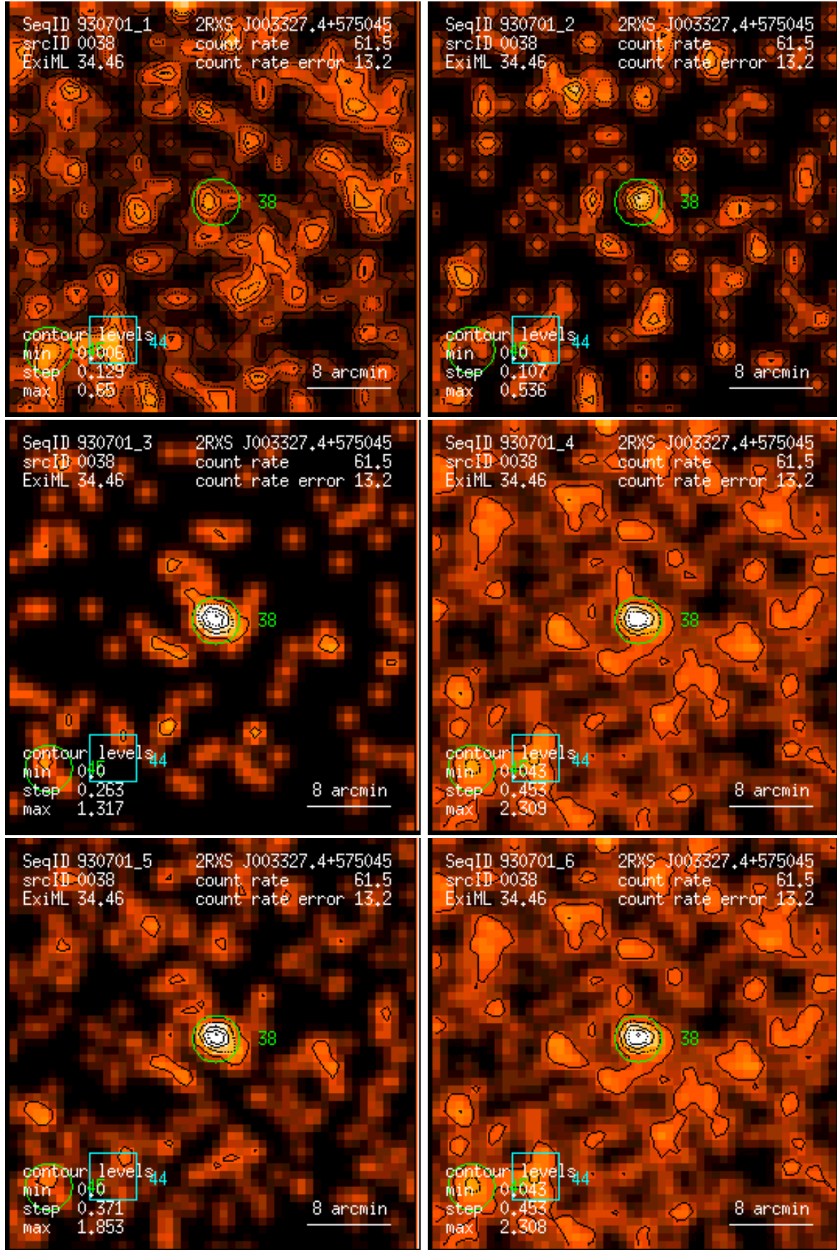
Figure 38: RASS 930701: detection 0038: band rate images, Gaussian filter: (1) PSPC channels 11 – 41, (2) 52 – 90, (3) 91 – 201, (4) 11 – 235, (5) 52 – 201, (6) 11 – 201. Broad band rates in counts/ks. Band rate contour levels in counts/ks/arcmin 2 .
