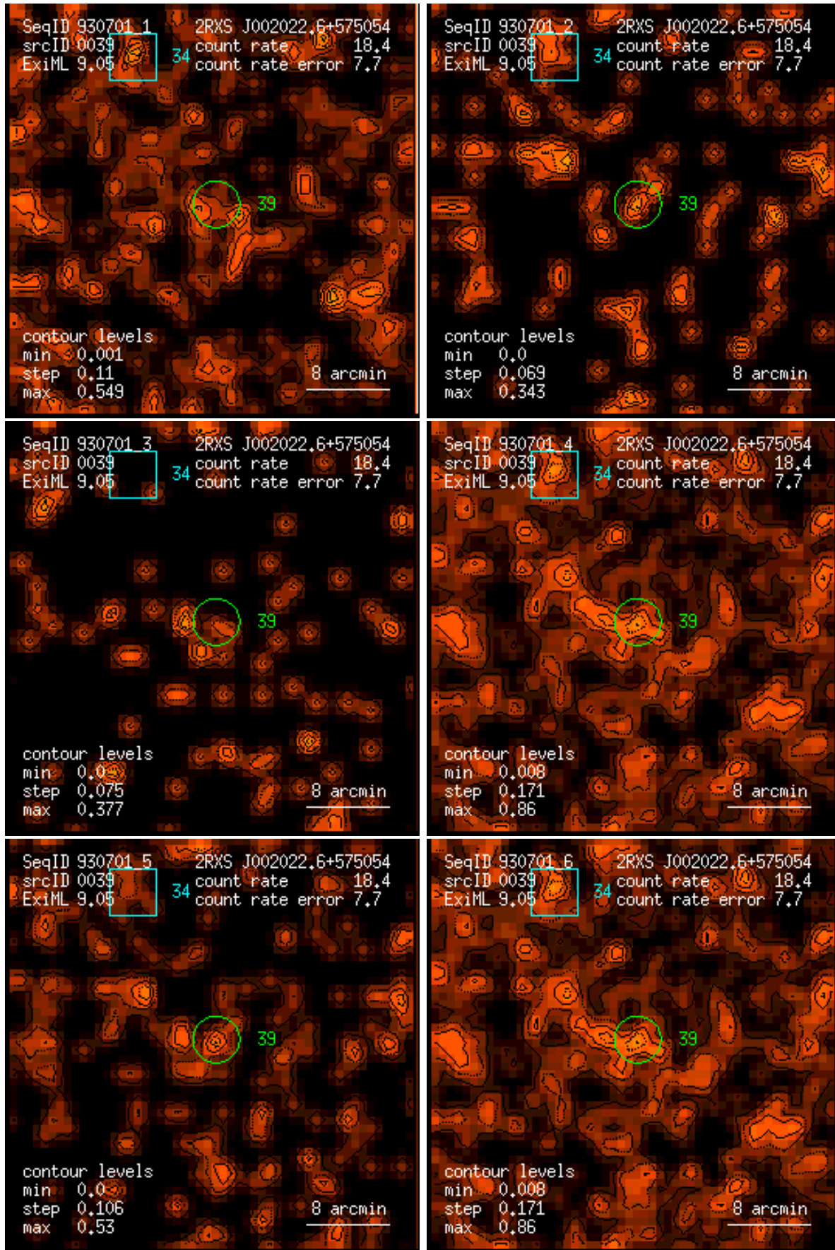
Figure 39: RASS 930701: detection 0039: band rate images, Gaussian filter: (1) PSPC channels 11 – 41, (2) 52 – 90, (3) 91 – 201, (4) 11 – 235, (5) 52 – 201, (6) 11 – 201. Broad band rates in counts/ks. Band rate contour levels in counts/ks/arcmin 2 .
