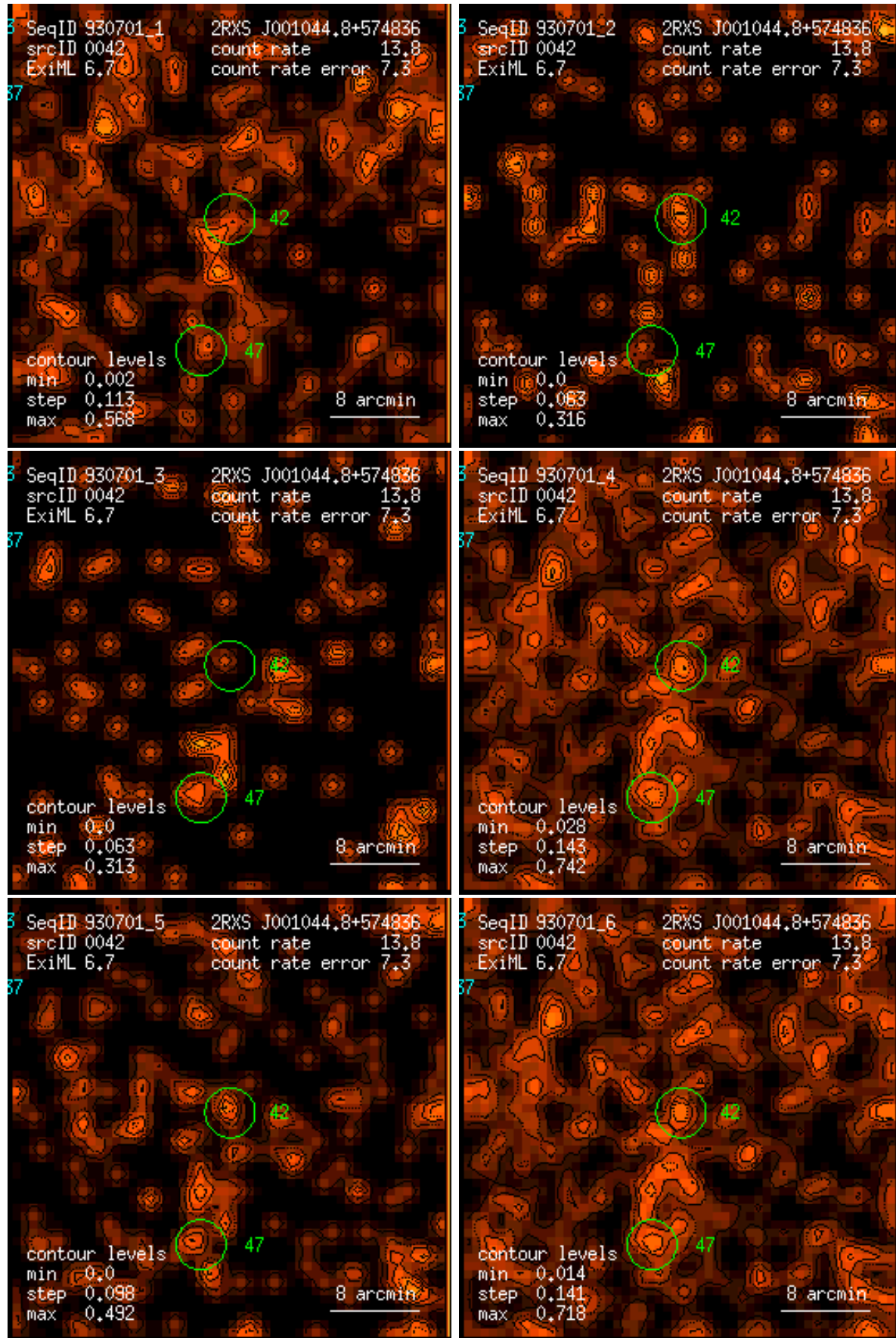
Figure 42: RASS 930701: detection 0042: band rate images, Gaussian filter: (1) PSPC channels 11 – 41, (2) 52 – 90, (3) 91 – 201, (4) 11 – 235, (5) 52 – 201, (6) 11 – 201. Broad band rates in counts/ks. Band rate contour levels in counts/ks/arcmin 2 .
