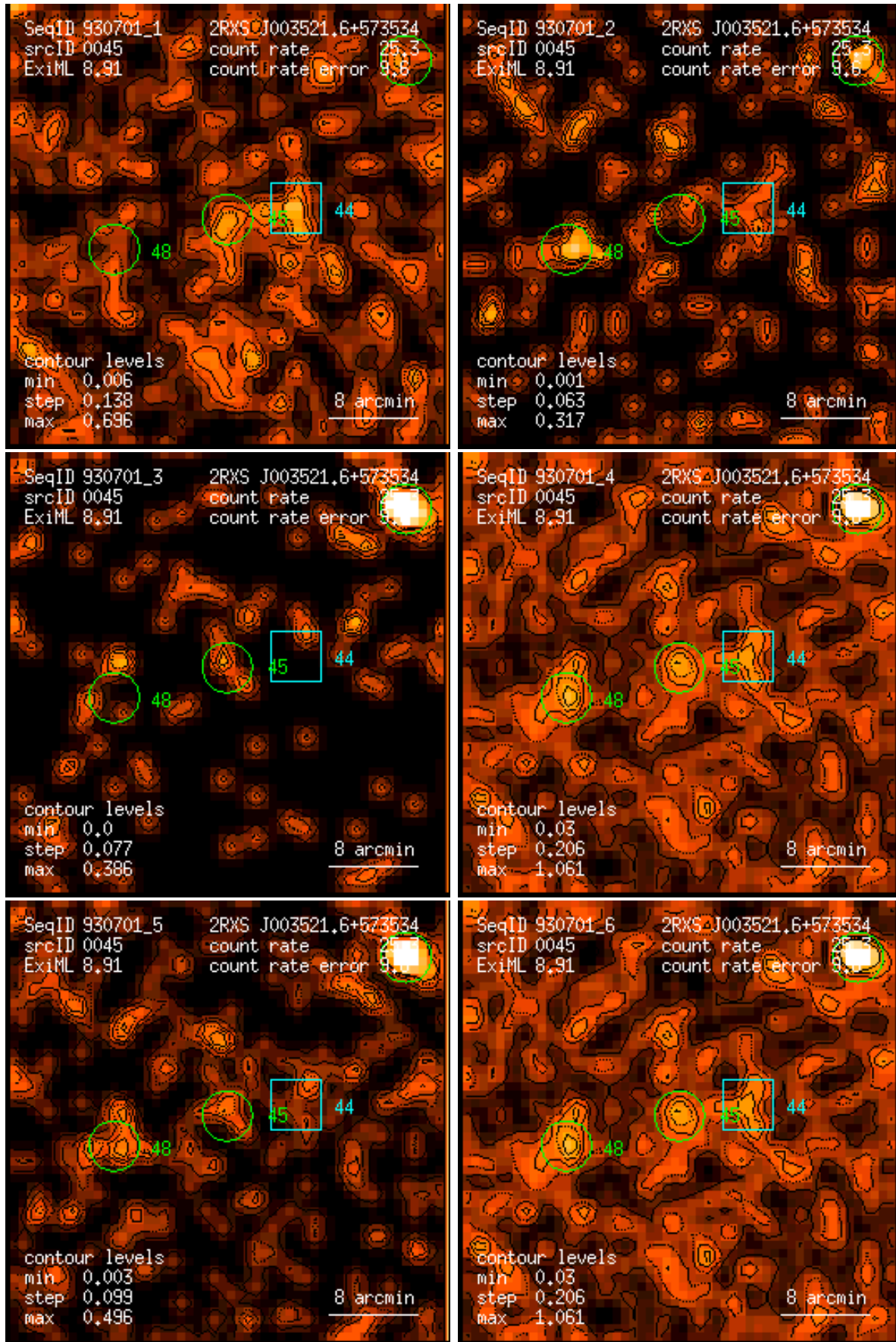
Figure 45: RASS 930701: detection 0045: band rate images, Gaussian filter: (1) PSPC channels 11 – 41, (2) 52 – 90, (3) 91 – 201, (4) 11 – 235, (5) 52 – 201, (6) 11 – 201. Broad band rates in counts/ks. Band rate contour levels in counts/ks/arcmin 2 .
