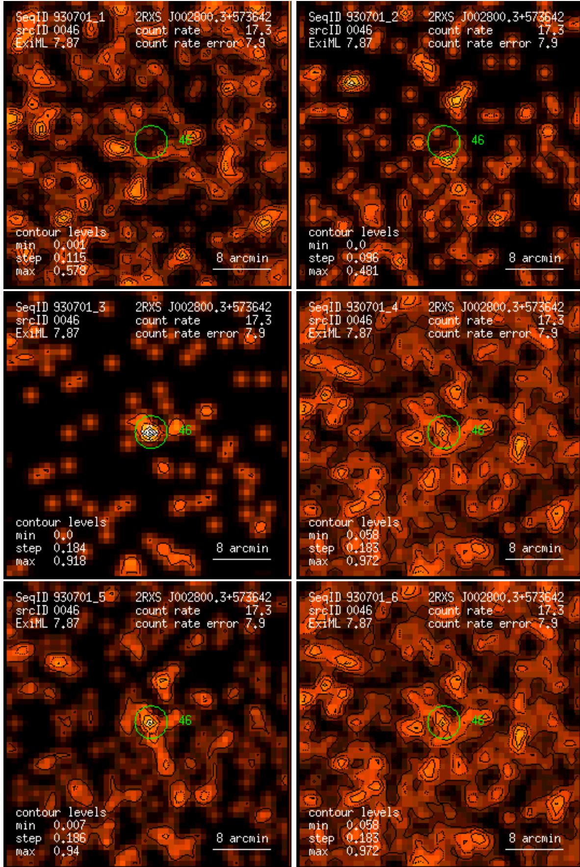
Figure 46: RASS 930701: detection 0046: band rate images, Gaussian filter: (1) PSPC channels 11 – 41, (2) 52 – 90, (3) 91 – 201, (4) 11 – 235, (5) 52 – 201, (6) 11 – 201. Broad band rates in counts/ks. Band rate contour levels in counts/ks/arcmin 2 .
