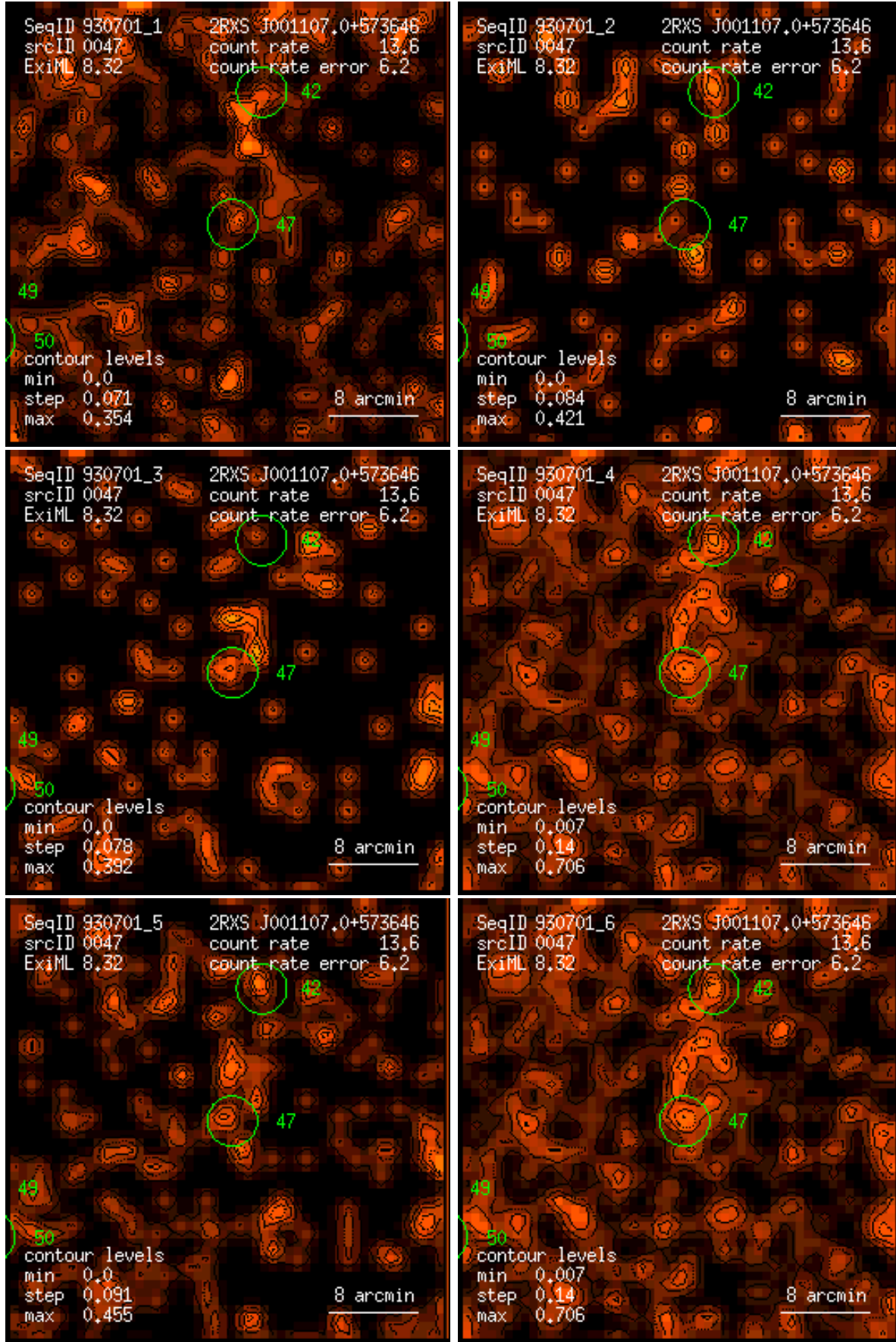
Figure 47: RASS 930701: detection 0047: band rate images, Gaussian filter: (1) PSPC channels 11 – 41, (2) 52 – 90, (3) 91 – 201, (4) 11 – 235, (5) 52 – 201, (6) 11 – 201. Broad band rates in counts/ks. Band rate contour levels in counts/ks/arcmin 2 .
