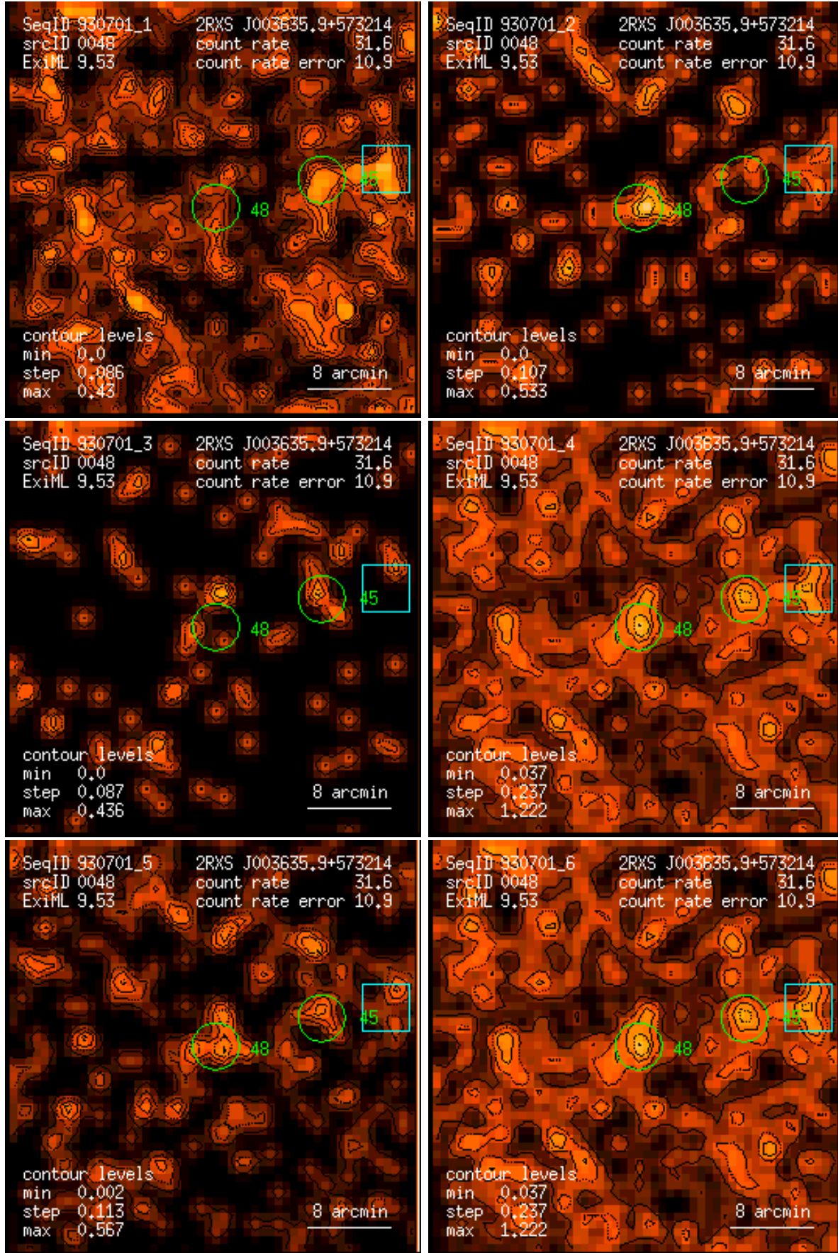
Figure 48: RASS 930701: detection 0048: band rate images, Gaussian filter: (1) PSPC channels 11 – 41, (2) 52 – 90, (3) 91 – 201, (4) 11 – 235, (5) 52 – 201, (6) 11 – 201. Broad band rates in counts/ks. Band rate contour levels in counts/ks/arcmin 2 .
