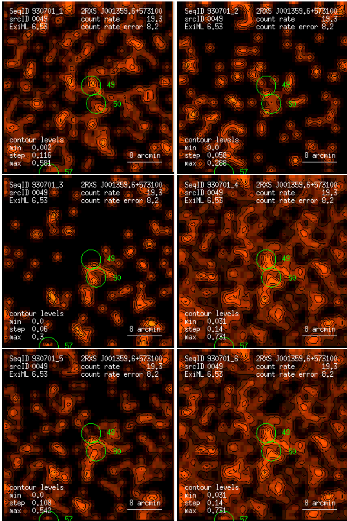
Figure 49: RASS 930701: detection 0049: band rate images, Gaussian filter: (1) PSPC channels 11 – 41, (2) 52 – 90, (3) 91 – 201, (4) 11 – 235, (5) 52 – 201, (6) 11 – 201. Broad band rates in counts/ks. Band rate contour levels in counts/ks/arcmin 2 .
