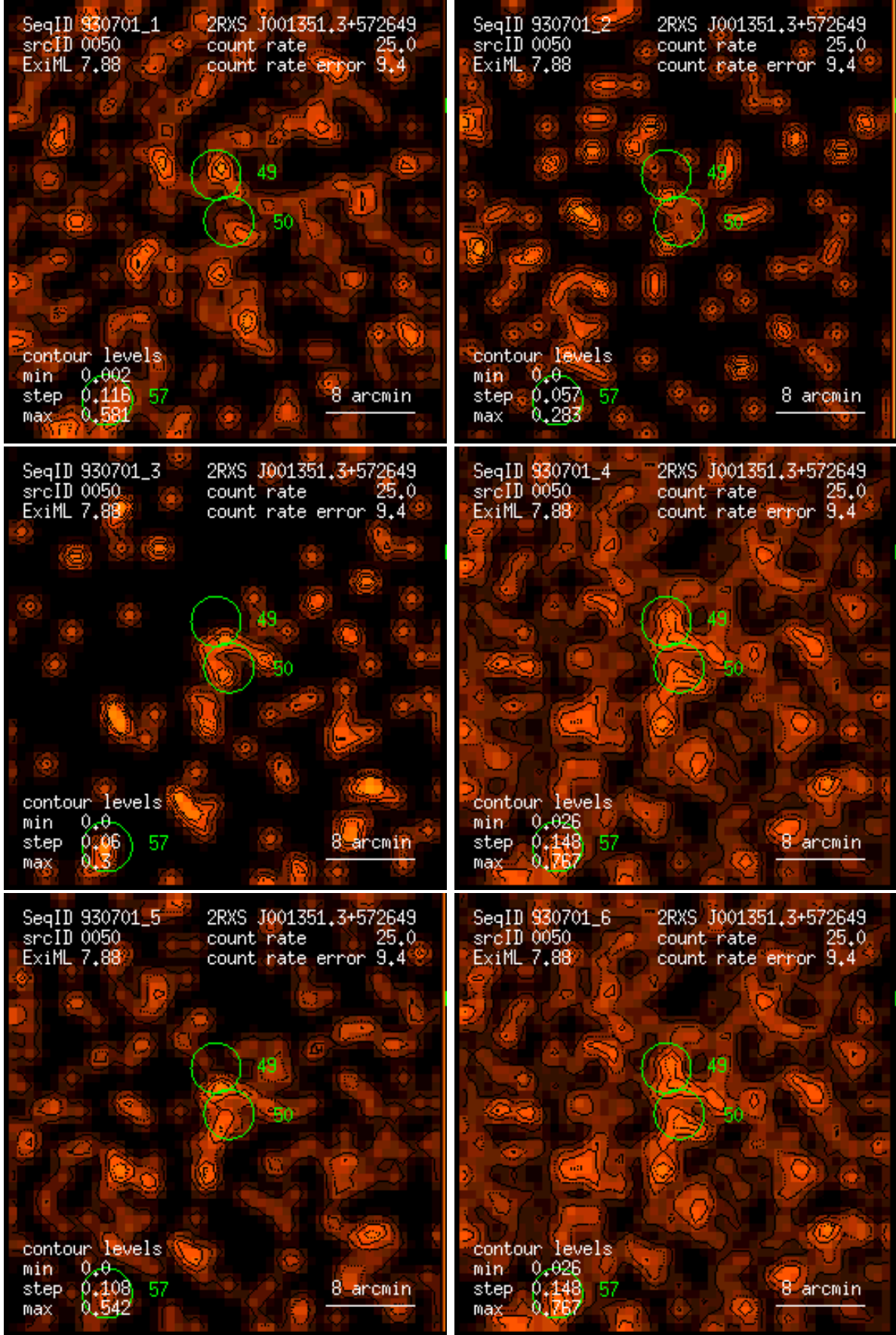
Figure 50: RASS 930701: detection 0050: band rate images, Gaussian filter: (1) PSPC channels 11 – 41, (2) 52 – 90, (3) 91 – 201, (4) 11 – 235, (5) 52 – 201, (6) 11 – 201. Broad band rates in counts/ks. Band rate contour levels in counts/ks/arcmin 2 .
