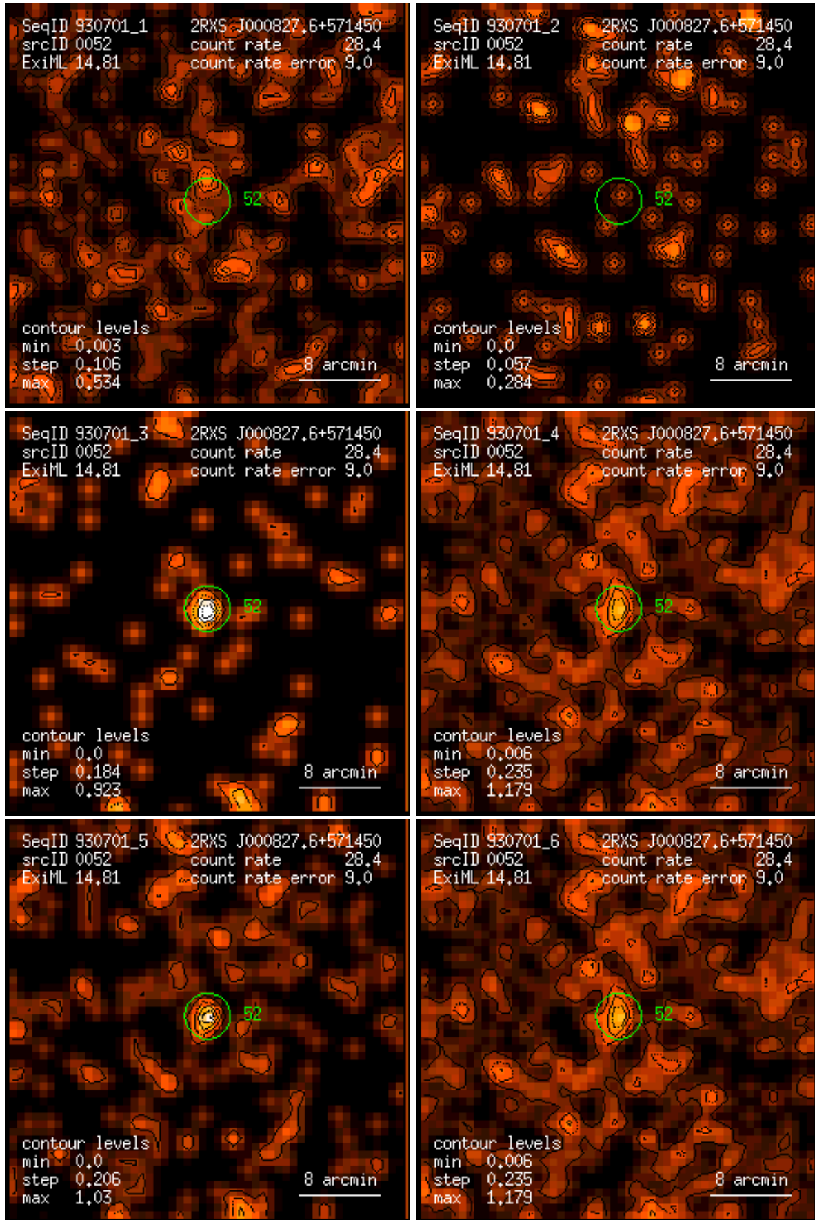
Figure 52: RASS 930701: detection 0052: band rate images, Gaussian filter: (1) PSPC channels 11 – 41, (2) 52 – 90, (3) 91 – 201, (4) 11 – 235, (5) 52 – 201, (6) 11 – 201. Broad band rates in counts/ks. Band rate contour levels in counts/ks/arcmin 2 .
