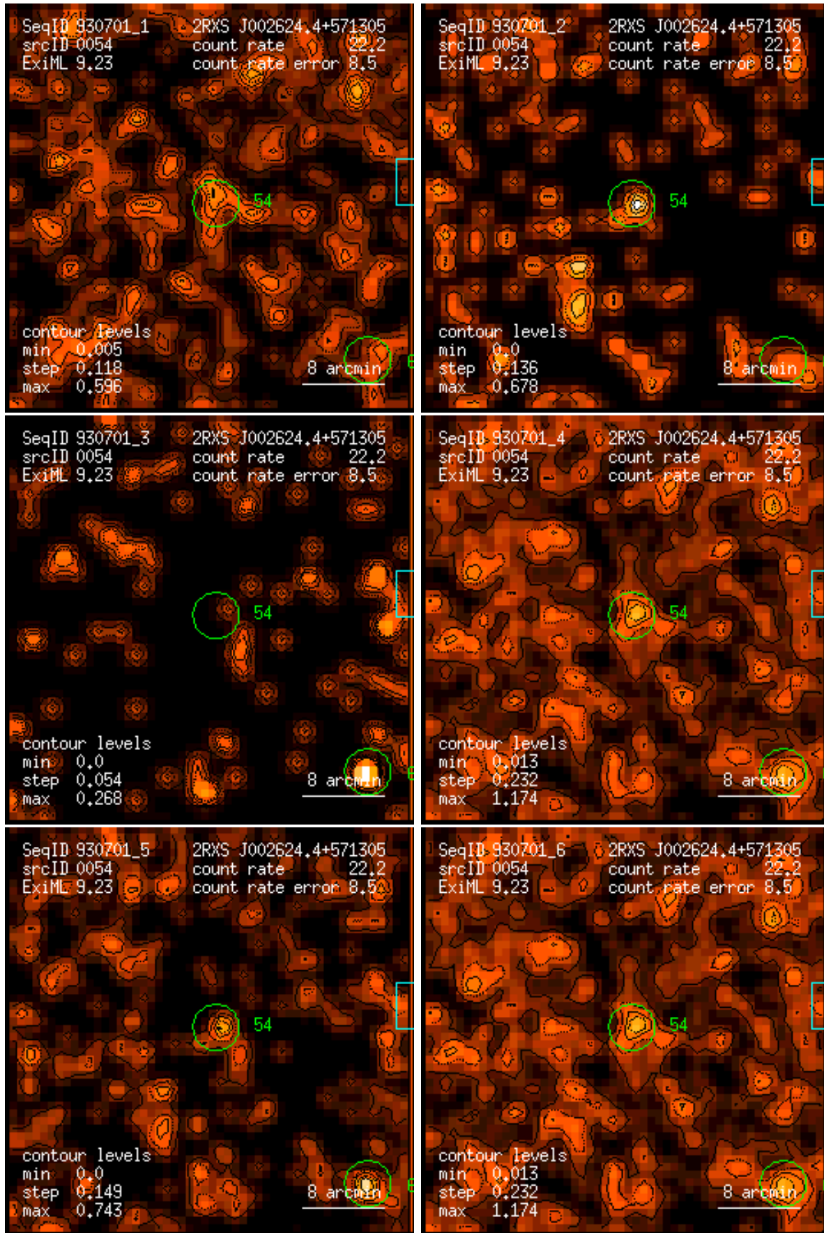
Figure 54: RASS 930701: detection 0054: band rate images, Gaussian filter: (1) PSPC channels 11 – 41, (2) 52 – 90, (3) 91 – 201, (4) 11 – 235, (5) 52 – 201, (6) 11 – 201. Broad band rates in counts/ks. Band rate contour levels in counts/ks/arcmin 2 .
