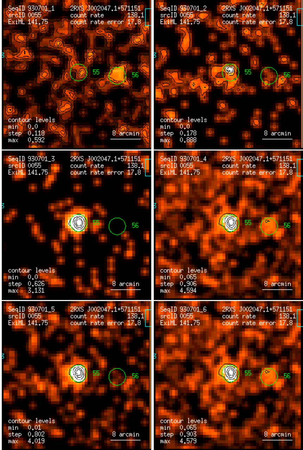
Figure 55: RASS 930701: detection 0055: band rate images, Gaussian filter: (1) PSPC channels 11 – 41, (2) 52 – 90, (3) 91 – 201, (4) 11 – 235, (5) 52 – 201, (6) 11 – 201. Broad band rates in counts/ks. Band rate contour levels in counts/ks/arcmin 2 .
