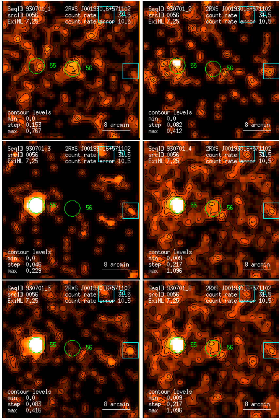
Figure 56: RASS 930701: detection 0056: band rate images, Gaussian filter: (1) PSPC channels 11 – 41, (2) 52 – 90, (3) 91 – 201, (4) 11 – 235, (5) 52 – 201, (6) 11 – 201. Broad band rates in counts/ks. Band rate contour levels in counts/ks/arcmin 2 .
