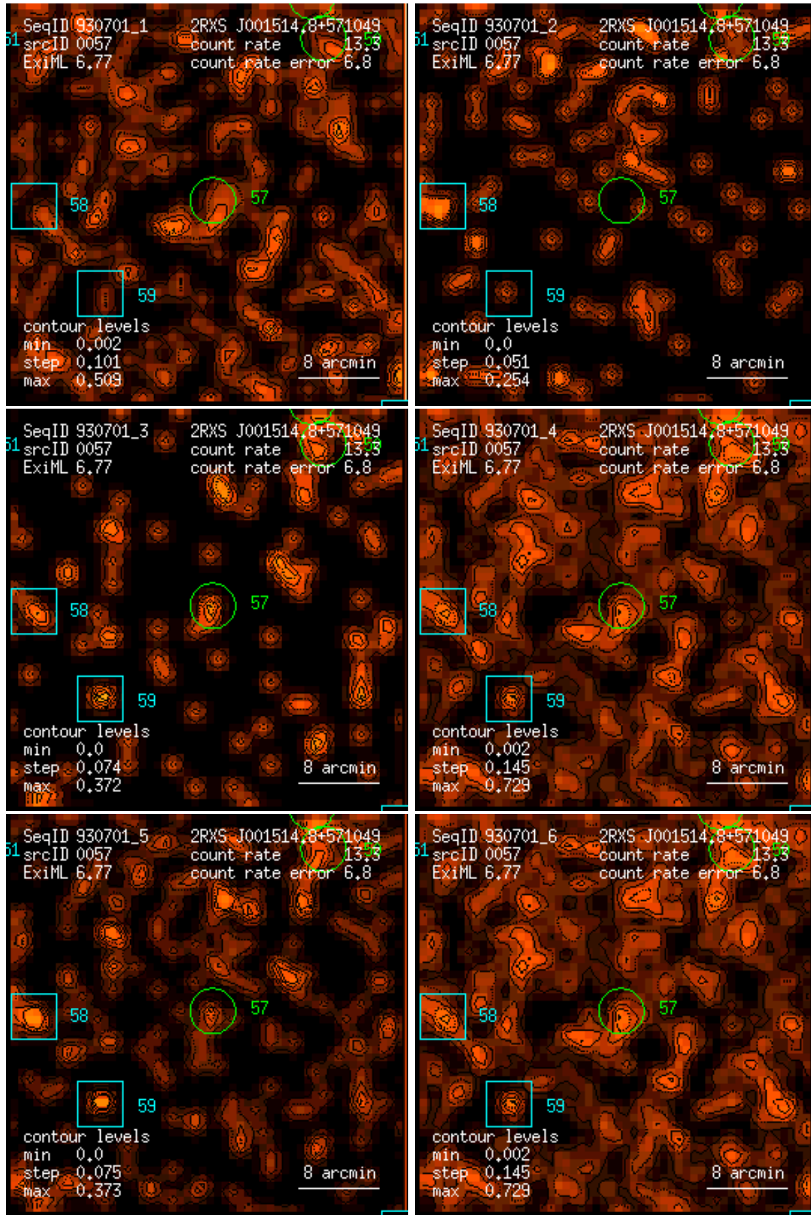
Figure 57: RASS 930701: detection 0057: band rate images, Gaussian filter: (1) PSPC channels 11 – 41, (2) 52 – 90, (3) 91 – 201, (4) 11 – 235, (5) 52 – 201, (6) 11 – 201. Broad band rates in counts/ks. Band rate contour levels in counts/ks/arcmin 2 .
