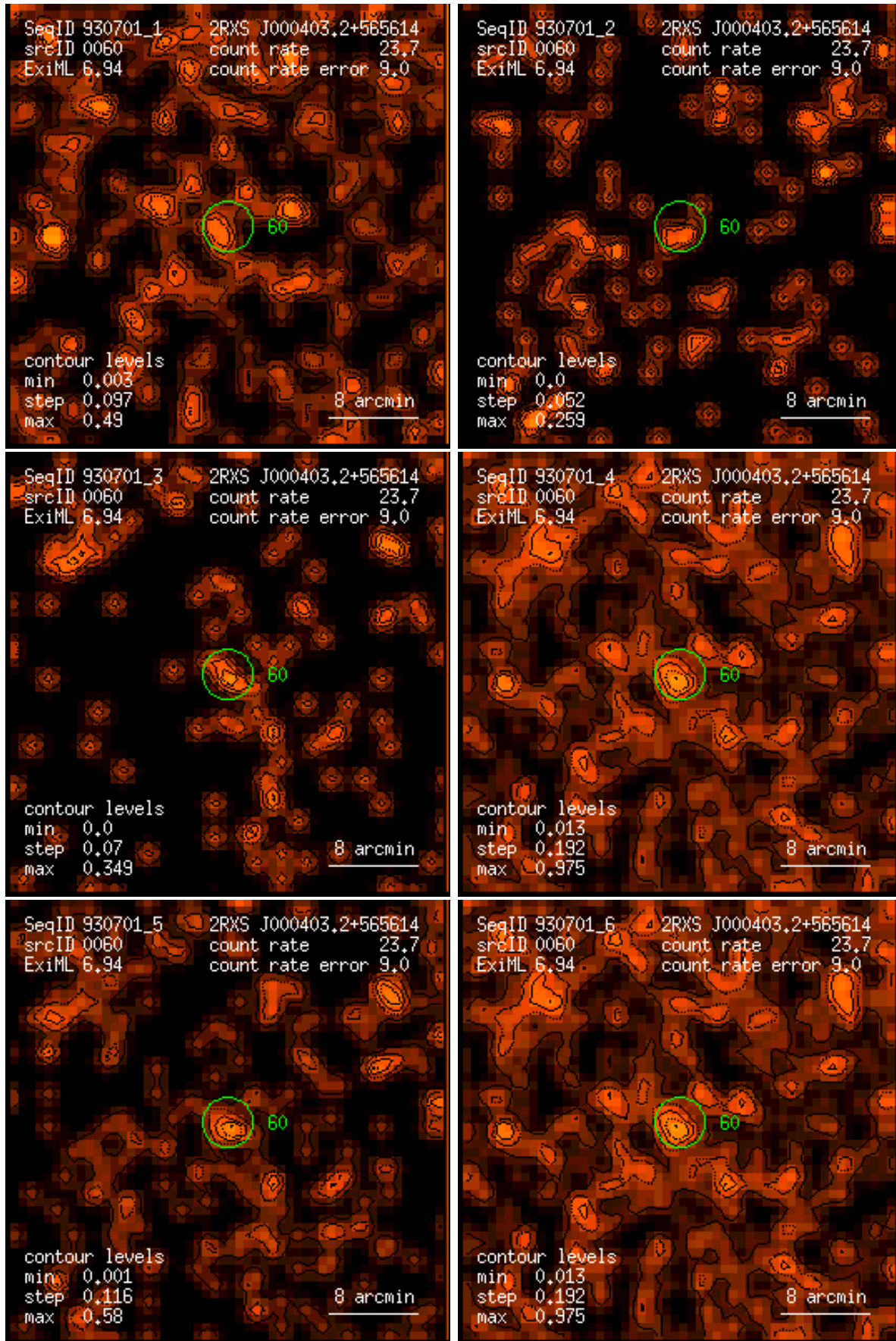
Figure 60: RASS 930701: detection 0060: band rate images, Gaussian filter: (1) PSPC channels 11 – 41, (2) 52 – 90, (3) 91 – 201, (4) 11 – 235, (5) 52 – 201, (6) 11 – 201. Broad band rates in counts/ks. Band rate contour levels in counts/ks/arcmin 2 .
