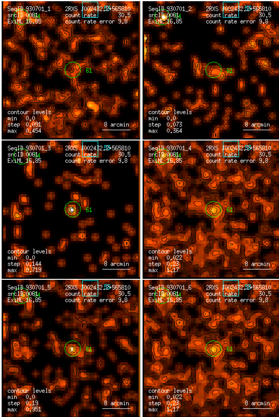
Figure 61: RASS 930701: detection 0061: band rate images, Gaussian filter: (1) PSPC channels 11 – 41, (2) 52 – 90, (3) 91 – 201, (4) 11 – 235, (5) 52 – 201, (6) 11 – 201. Broad band rates in counts/ks. Band rate contour levels in counts/ks/arcmin 2 .
