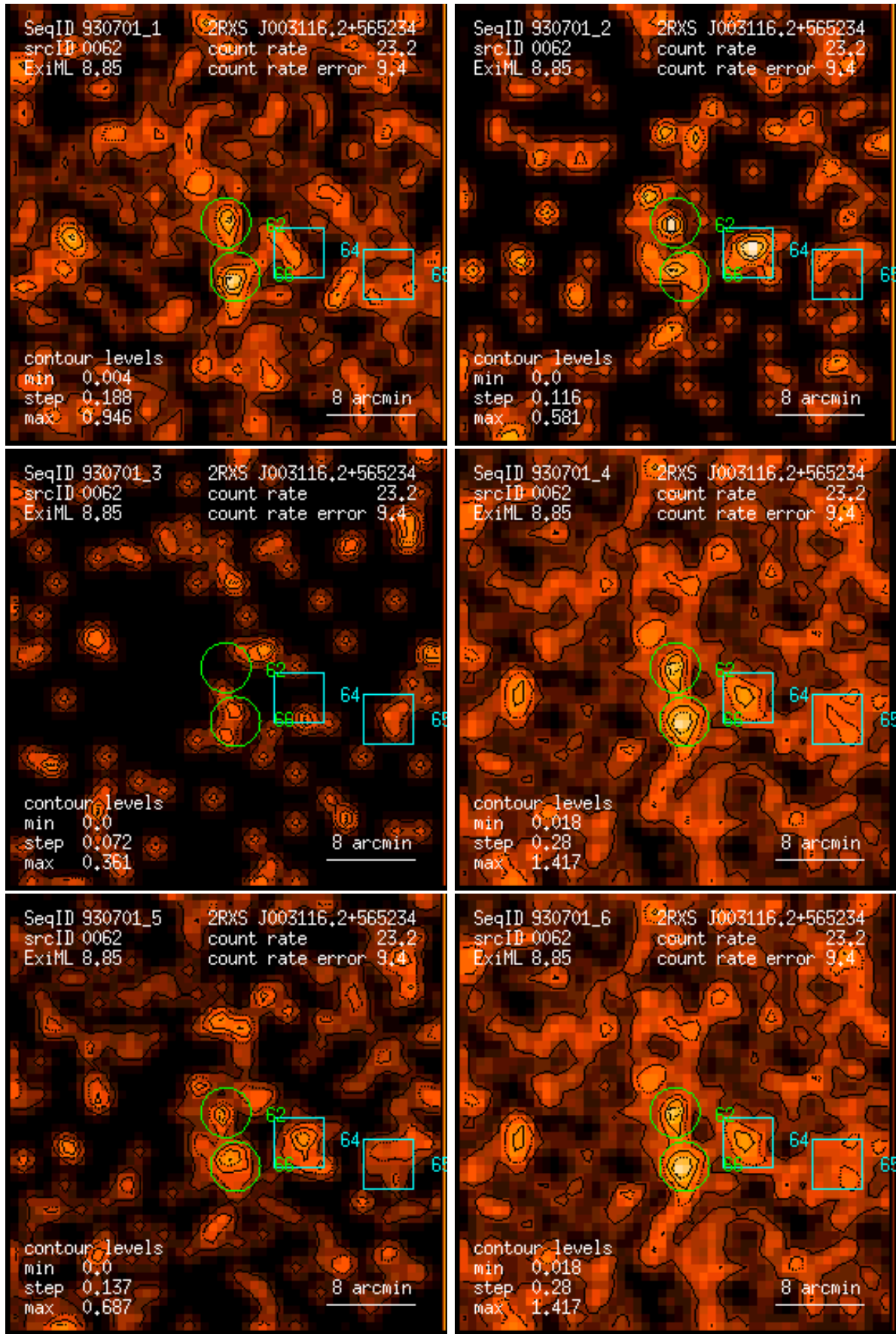
Figure 62: RASS 930701: detection 0062: band rate images, Gaussian filter: (1) PSPC channels 11 – 41, (2) 52 – 90, (3) 91 – 201, (4) 11 – 235, (5) 52 – 201, (6) 11 – 201. Broad band rates in counts/ks. Band rate contour levels in counts/ks/arcmin 2 .
