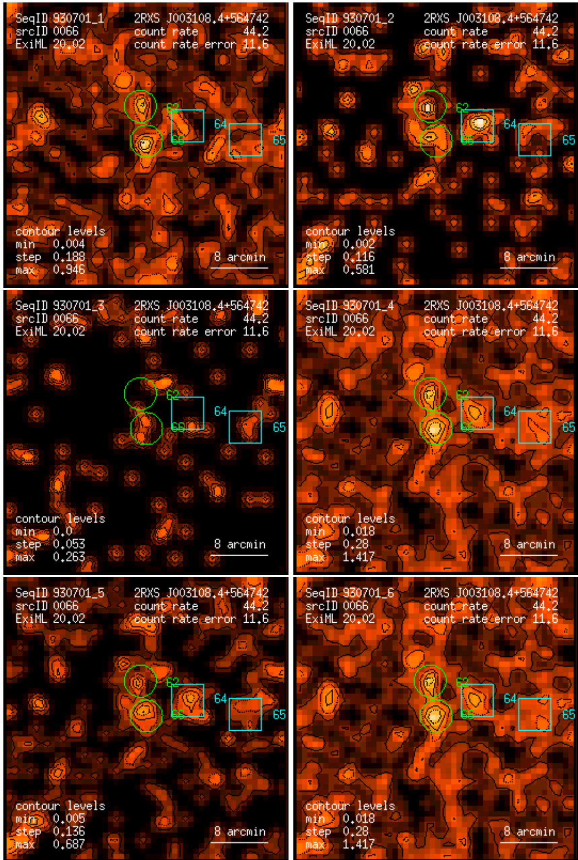
Figure 66: RASS 930701: detection 0066: band rate images, Gaussian filter: (1) PSPC channels 11 – 41, (2) 52 – 90, (3) 91 – 201, (4) 11 – 235, (5) 52 – 201, (6) 11 – 201. Broad band rates in counts/ks. Band rate contour levels in counts/ks/arcmin 2 .
